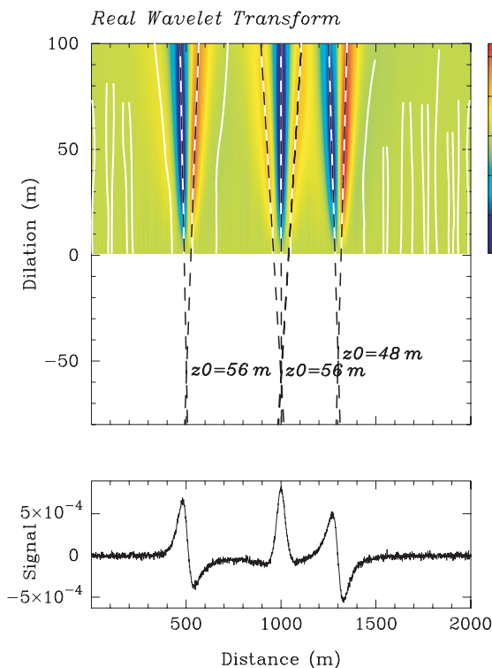
Figure 2. Real multiscale tomography (RMST). Bottom: Noisy synthetic magnetic intensity generated by three magnetic dipoles of different inclination ( 30^\circ , 90^\circ and 0^\circ ) located in the subsurface earth at depth z = 50 m and lateral distances 500, 1000 and 1250 m, respectively. Top: Amplitude of the RMST. The intersection of the lines of extrema (extrema of energy of the real wavelet transform) allows to localize each source depth (or dilation z ). The depths obtained are in good agreement to the true depths (56, 56 and 48 m).
