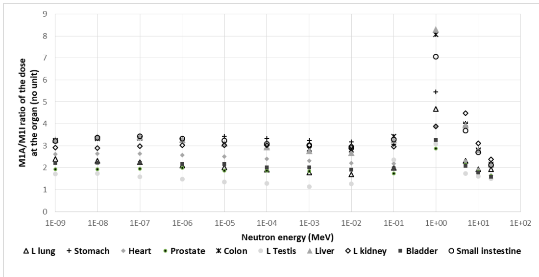
Figure 17. Ratio of the dose at the organ for the M1A phantom divided by the dose at the organ for the M1I phantom, for different organs, and as a function of the neutron energy.
