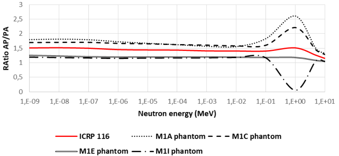
Figure 3. AP/PA ratio of the conversion coefficients for the ICRP report (red curves) and AP/PA ratio of the organ doses for the liver estimated in our calculations with 4 different phantoms (4 black curves).
