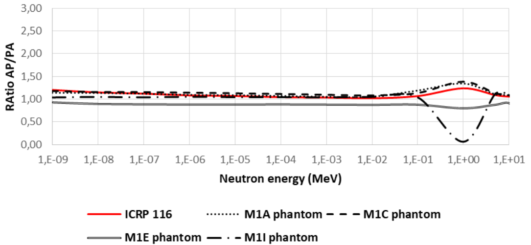
Figure 4. AP/PA ratio of the conversion coefficients for the ICRP report (red curves) and AP/PA ratio of the organ doses for the lung estimated in our calculations with 4 different phantoms (4 black curves).
