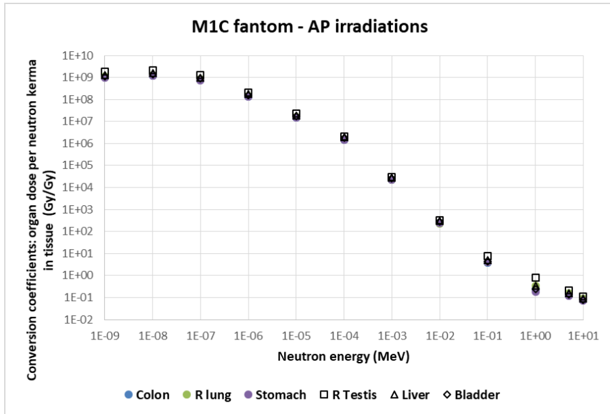
Figure 12. Conversion coefficients for the M1C phantom for a neutron source at 0°.
