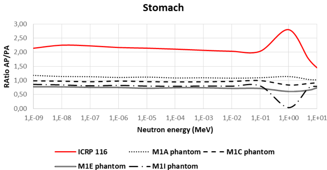
Figure 6. AP/PA ratio of the conversion coefficients for the ICRP report (red curves) and AP/PA ratio of the organ doses for the stomach estimated in our calculations with 4 different phantoms (4 black curves).
