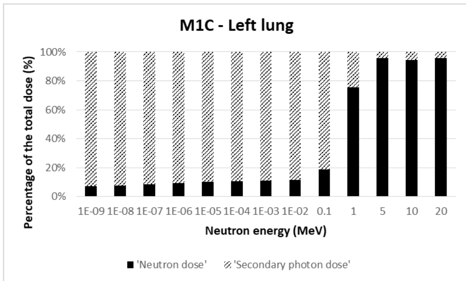
Figure 13. Contribution of the dose as a function of types of secondary particles, for the left lung, for the phantom M1C with an incidence of 0°.
