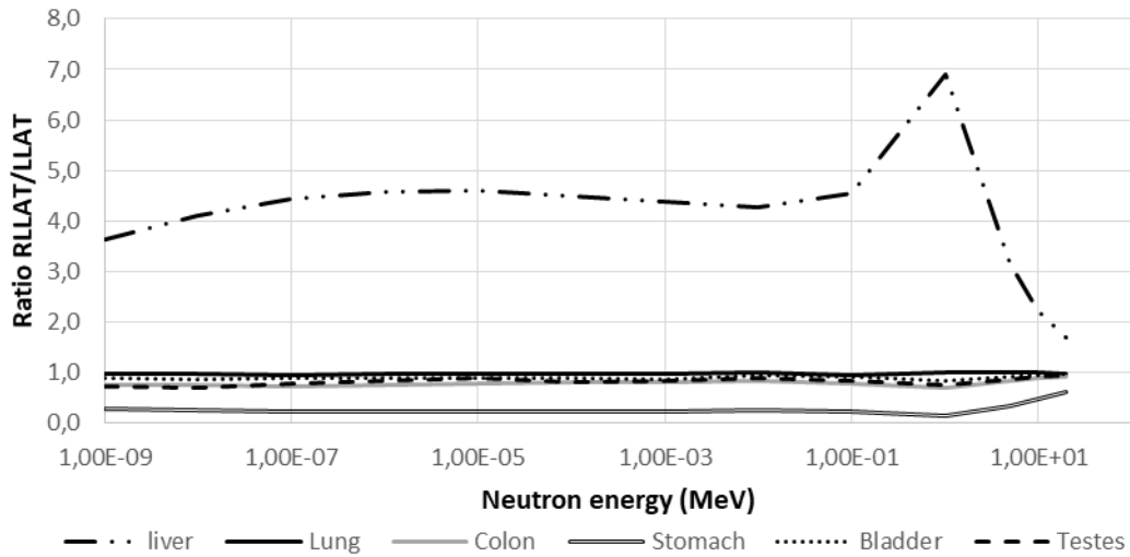
Figure 8. RLAT/LLAT ratios of the conversion coefficients as a function of neutron energy, for different organs, for the ICRP phantom.
