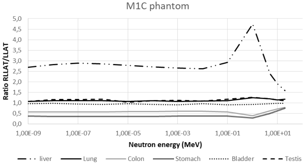
Figure 10. RLAT/LLAT ratios of the conversion coefficients as a function of neutron energy, for different organs, for the M1C phantom.
