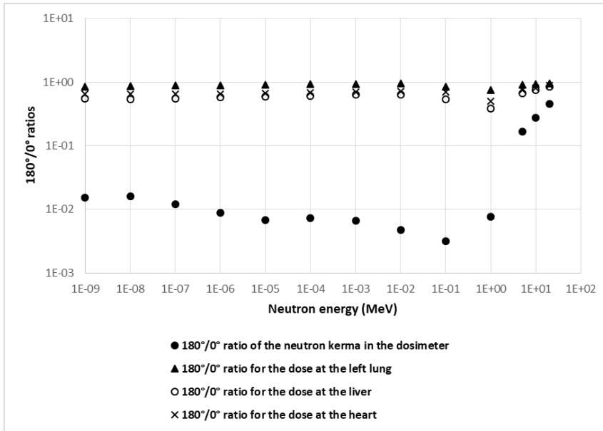
Figure 16. PA/AP ratios of the neutron kerma in tissue and for different doses at the organs, for the M1A phantom.
