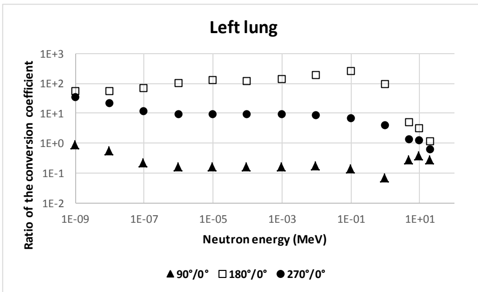
Figure 15. Ratio of the coefficients for the 90° or 180° or 270° of incidence divided by the 0° one, for the M1A phantom for the left lung.
