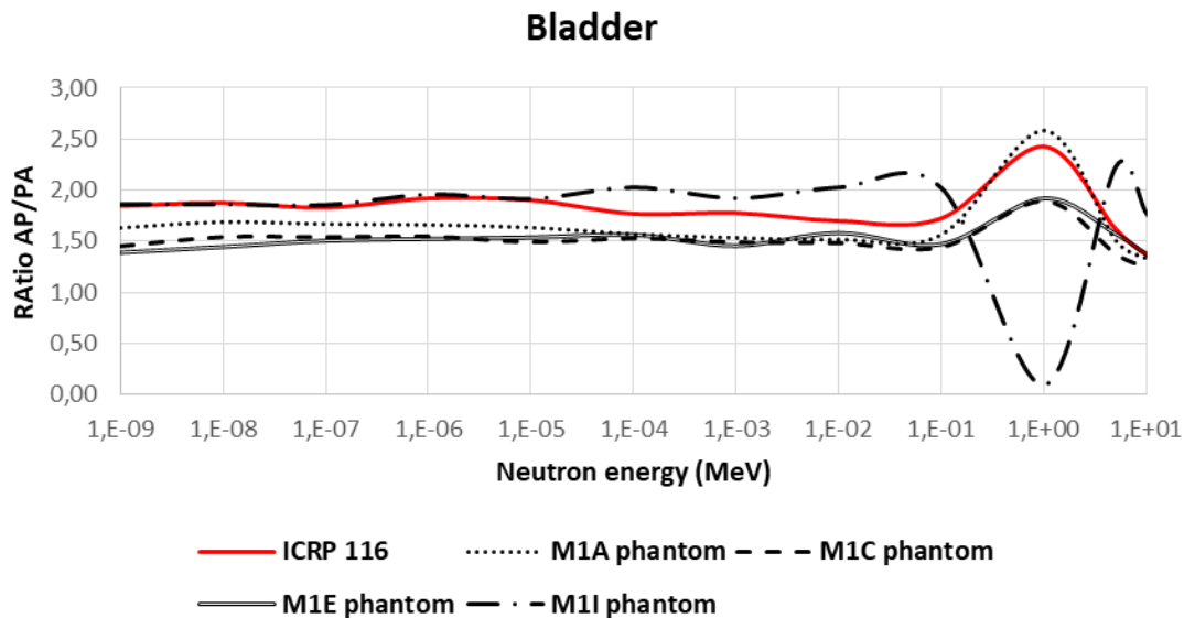
Figure 5. AP/PA ratio of the conversion coefficients for the ICRP report (red curves) and AP/PA ratio of the organ doses for the bladder estimated in our calculations with 4 different phantoms (4 black curves).
