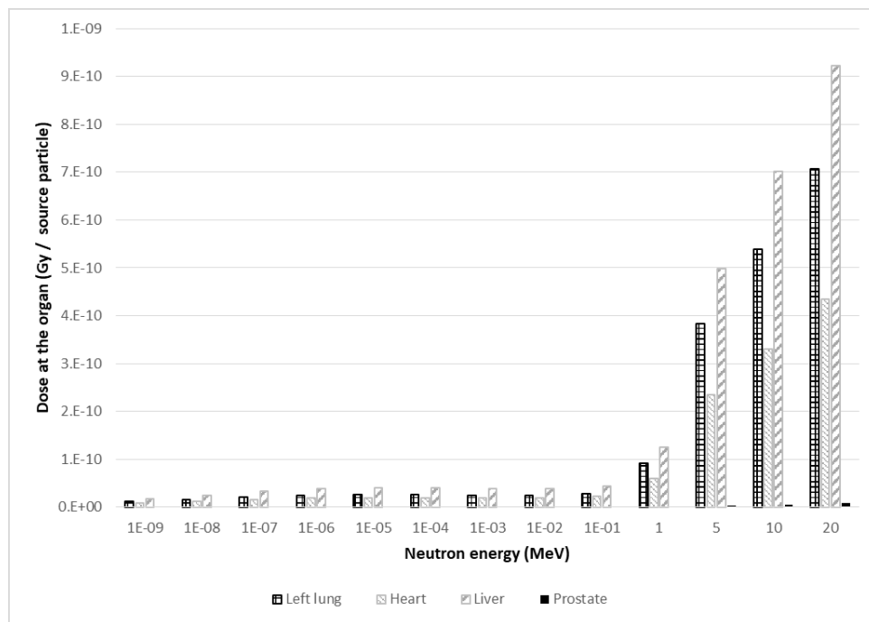
Figure 14. Dose for four different organs for the M1C phantom with an incidence of 0°.
