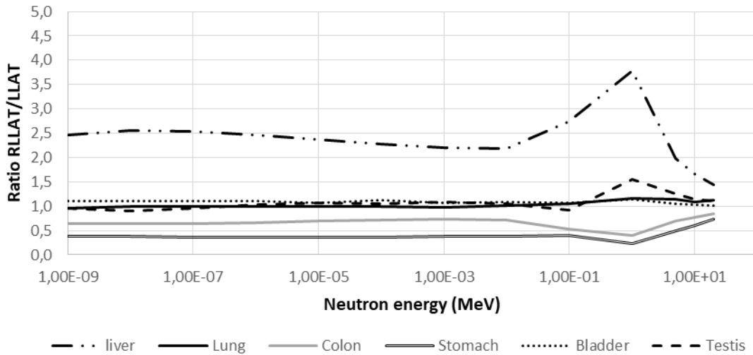
Figure 9. RLAT/LLAT ratios of the conversion coefficients as a function of neutron energy, for different organs, for the M1A phantom.
