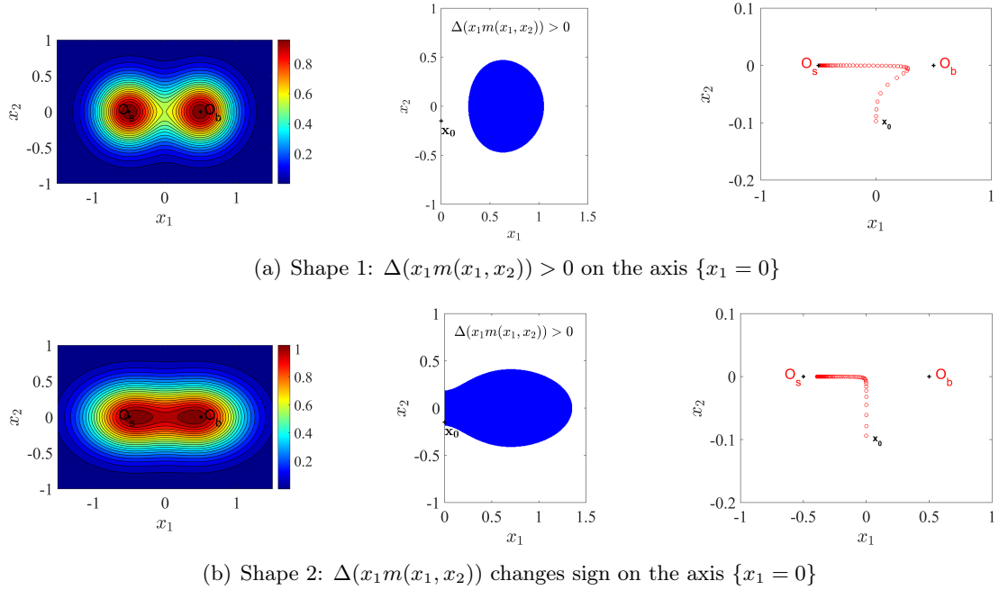
Figure 3: Trajectory of adaptation with different shapes of the fitness function. The left panels depict the fitness function. The central panels describe the sign of \Delta(x_1 m(x_1, x_2)) in the region \{x_1 > 0\} : this quantity is negative in the blue region and positive otherwise. The right panels depict the corresponding trajectories of the mean phenotype \bar{\mathbf{x}}(t) obtained with the model (\mathcal{Q}_b) , at successive times t = 0, 1, \dots, 100 . In both cases, the initial condition is concentrated at \mathbf{x}_0 = (0, -0.1) , leading to a positive sign of \Delta(x_1 m(x_1, x_2)) at (x_1, x_2) = \mathbf{x}_0 in the upper panels and a negative sign in the lower panels. The parameter values are the same as in Fig. 2, except for the fitness function of the lower panel, where \sigma_{x_1}^2 = 1/18 and \sigma_{x_2}^2 = 1/10 .
