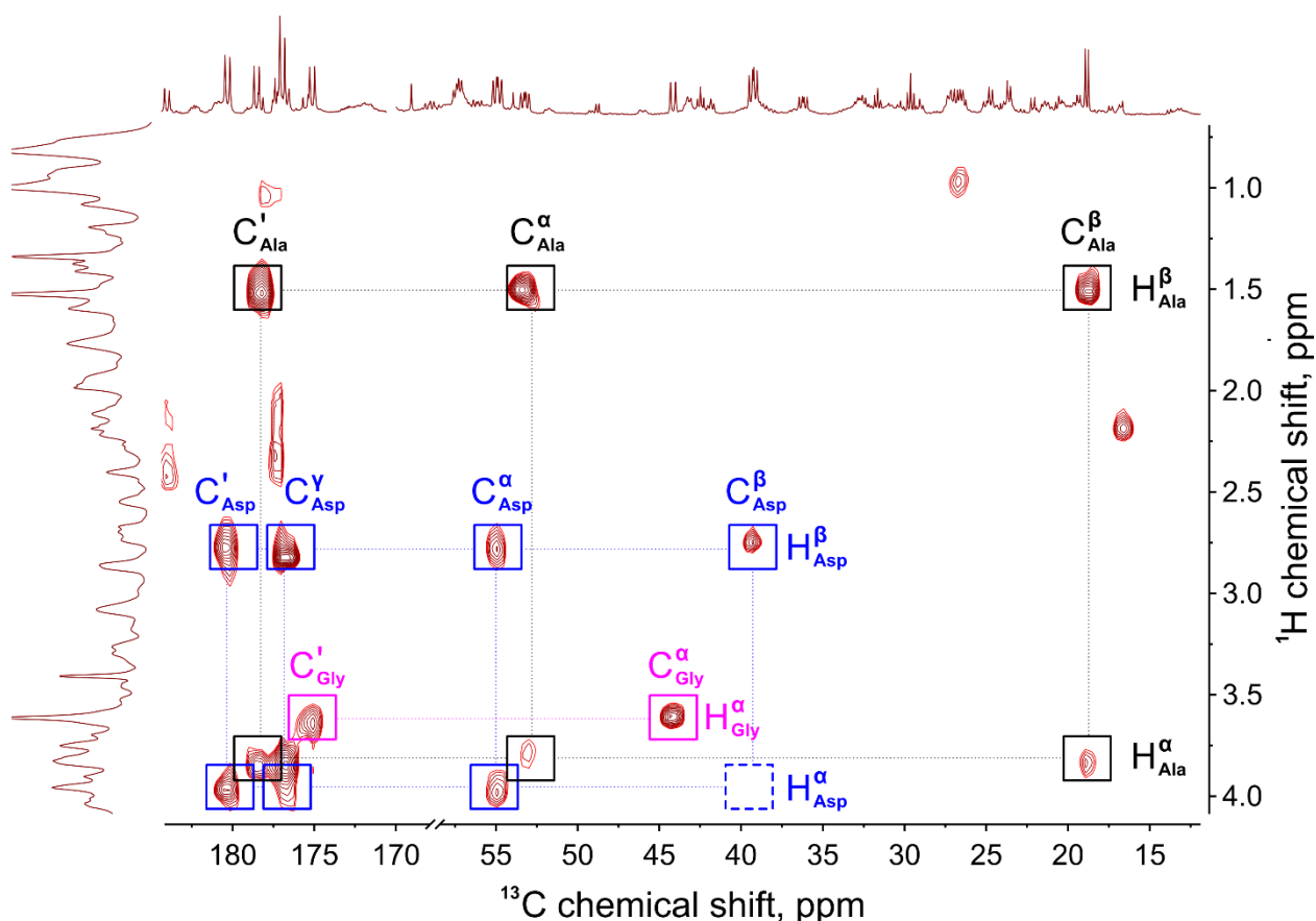
Figure 4. ZULF-TOCSY spectrum of the ISOGRO supernatant in D_2O (pH=6.5). Experimental parameters: B_{UL} = 50 nT, t_{mix} = 40 ms, 64 transients in indirect direction, 960 scans per transient, relaxation delay 3 s, total experiment duration ca. 69 hours.
