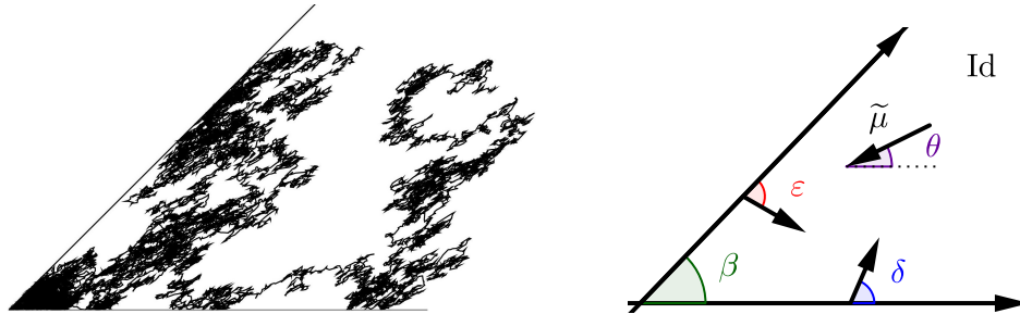
FIGURE 1. A trajectory of the reflected Brownian motion in a wedge, and the parameters \beta , \tilde{\mu} , \theta , \delta and \varepsilon .
