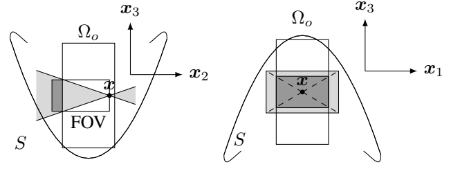
Fig. 6. An example FOV not suitable for the M-line method, because the (two) cones of lines (light grey) from \boldsymbol{x} which intersect \text{FOV} \setminus \Omega_o (dark grey) do not intersect the saddle trajectory S . Therefore there can be no M-line that intersects \text{FOV} \setminus \Omega_o , and reconstruction inside all \text{FOV} \cap \Omega_o cannot be performed using the M-line method.
