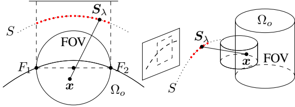
Fig. 12. Top view (left) and side view (right) for a semicircular FOV with an M-line from S_\lambda and passing through x . The red dotted curve is the part of the source trajectory S whose projection intersects the projection of the FOV. For each point x of \Omega_o \cap FOV \cap C_S , every M-line from a source position S_\lambda from the red part of the source trajectory S is suitable. Right: the dashed rectangle is the projection of the FOV onto a plane parallel to the vertical plane containing F_1 and F_2 . The dashed curve is the projection of the trajectory S .
