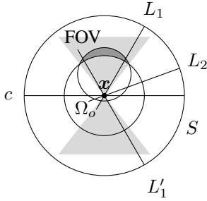
Fig. 5. Top view of a saddle trajectory S and an object with support \Omega_o . Here, \boldsymbol{x} is on the chord c and the DBP method cannot be directly applied, because c \cap \text{FOV} is in the strict interior of c \cap \Omega_o , see [10]. However, M-line method can be applied here. L_1 is a suitable M-line, because L_1 \cap \Omega_F \neq \emptyset ( \Omega_F = \text{FOV} \setminus \Omega_o is the dark grey region). Similarly for L'_1 but not for L_2 (see [10] and [4]). The grey cones delimit the suitable M-lines.
