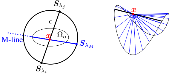
Fig. 4. Left : Top view of a chord c and an M-line from S_{\lambda_M} . Right : Parts of some M-lines (in blue) through a point \boldsymbol{x} which is inside the convex hull C_S of the saddle trajectory. A chord (in black) contains \boldsymbol{x} .
