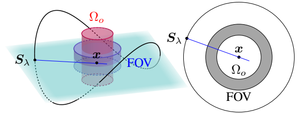
Fig. 7. A saddle trajectory with only axial truncation. Considering a horizontal plane through \boldsymbol{x} \in \Omega_o \cap C_S \cap \text{FOV} , it is possible to have a suitable M-line (in blue) from an intersection between the horizontal plane and the trajectory. Right : top view, the dark grey annulus is \Omega_F .
