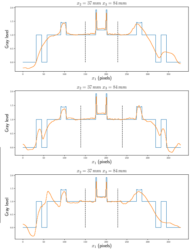
Fig. 15. Profiles from the reconstructions after 260 iterations at x_2 = 37 mm and x_3 = 84 mm (see Fig.13) for FOV1 (top), FOV2 (middle), FOV3 (bottom). The black dashed lines define the limits of the FOV.
