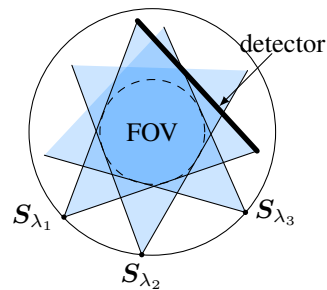
Fig. 2. The FOV defined as the intersection of the X-ray cones (here we show a 2D version, with three source positions). With the saddle trajectory, it is impossible to perfectly define a cylindrical FOV using a rectangular detector, but for simplicity we investigate a cylinder inside this FOV.
