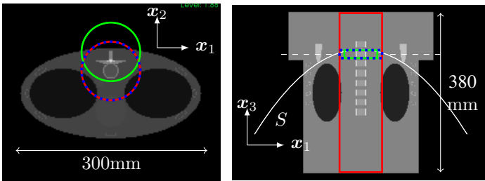
Fig. 13. Forbild thorax phantom in top view ( left ) and side view ( right ). FOV1 is represented by the blue dotted line, FOV2 is the red line and FOV3 is the green line. The white dashed line in the image at right corresponds to the profiles plot in Fig. 15. It can be seen on the right image that the projection (of the top) of FOV3 on a plane orthogonal to x_2 intersects the projection of S , thus making it type 2 sufficient.
