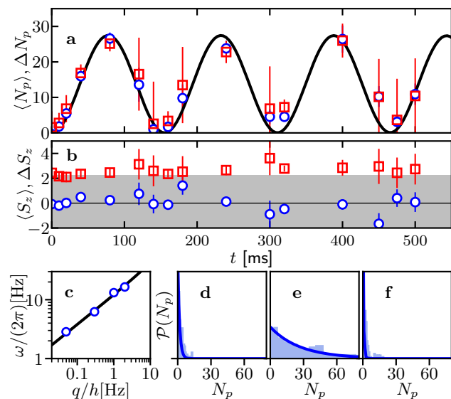
FIG. 1. Experimental observation of many-body oscillations. (a): Evolution of the mean number of pairs (circles) and its standard deviation (squares) in a sudden quench from q_i = 277 (3) Hz to q_f = 0.31 (1) Hz. Here N \approx 5400 (740). The solid line is the result of a fit of the Bogoliubov prediction (6) to the experimental data, with U_s = 17.5 (1.4) Hz as a single free parameter. (b): Mean (circles) and standard deviation (squares) of the magnetization S_z . The shaded region indicates the detection noise level. (c) Oscillation frequency obtained from a fit to the measured \bar{N}_p(t) (circles) for various q , compared to the prediction (5) (line). (d-f) Measured distribution of the number of pairs for t = 10, 80, 160 ms, with the solid lines corresponding to the prediction (7).
