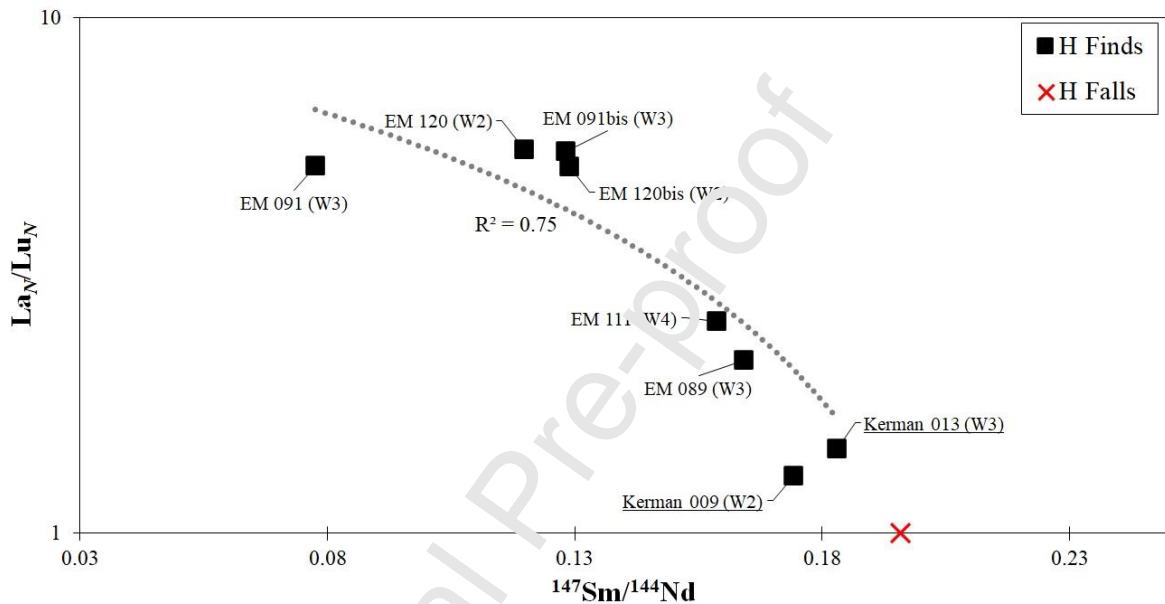
Fig. 6: ^{147}\text{Sm}/^{144}\text{Nd} versus La_N/Lu_N of the analyzed hot deserts compared to the fall ordinary chondrites. Samples from Lut are underlined. Dashed curve shows linear trend pattern of H finds. Standard deviation for ^{147}\text{Sm}/^{144}\text{Nd} of H falls in 0.0012 (n=10). Average elemental and isotopic ordinary chondrite values are from (Wasson and Kallemeyn, 1988) and (Bouvier et al., 2008), respectively.
