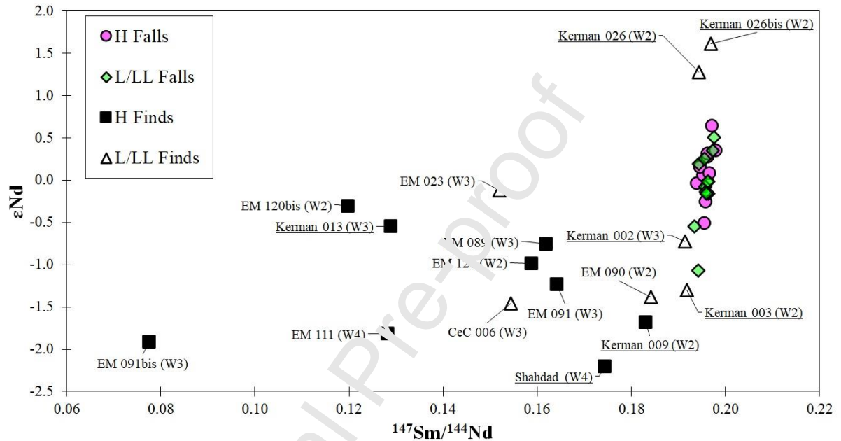
Fig. 3: ^{147}\text{Sm}/^{144}\text{Nd} versus \epsilon_{Nd} of the analyzed hot deserts compared to the fall ordinary chondrites. El Médano (EM) and Caleta el Cobre (CeC) are from the Atacama Desert. Kerman and Shahdad are from the Lut Desert (underlined). Data for fall ordinary chondrites are from (Bouvier et al., 2008).
