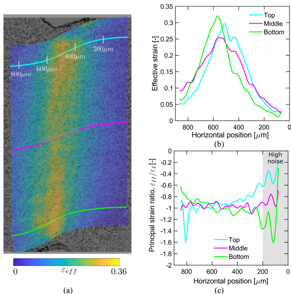
Fig. 9. Projection DIC strain field at step 6 (920N) right before onset of fracture. (a) Effective strain field highlighting the three lines at the top (cyan), middle (magenta) and bottom (green) of the gauge section. Line profiles of the effective strain (b) and the principal strain ratio (c) showing the loading state throughout the specimen. (For interpretation of the references to color in this figure legend, the reader is referred to the web version of this article.)
