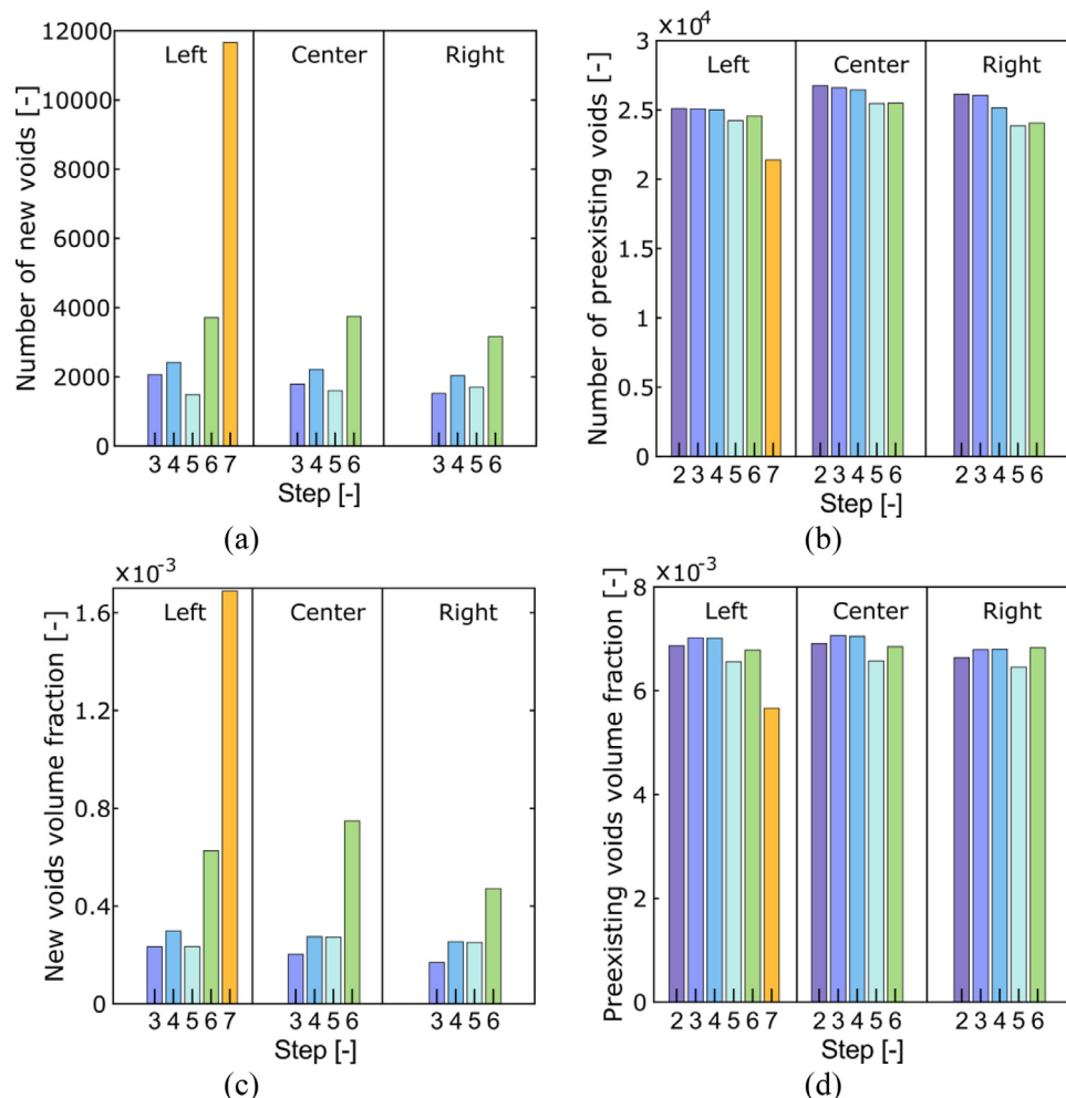
Fig. 12. Evolution of the pre-existing and new voids throughout the loading. The voids are tracked on the three large bins covering the gauge section (compare Fig. 5). (a) and (b) shows the evolution of the voids number while (c) and (d) shows the void volume fraction.
