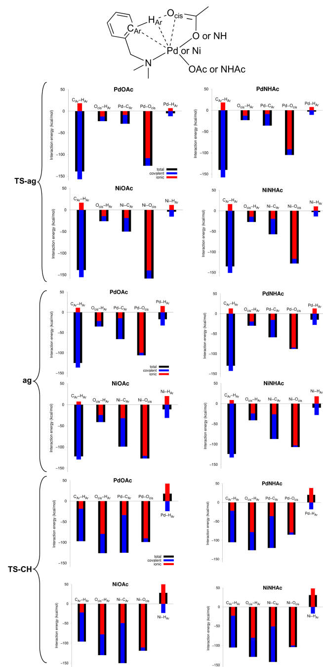
Figure 3. IQA analysis of TS-ag , ag and TS-CH in PdOAc , PdNHAc , NiOAc , NiNHAc systems. Histogram of atom-pair interaction energies within the reactive site (black coloured, total E_{\text{int}} in kcal/mol) are decomposed into their covalent component (blue coloured bars) and ionic component (red coloured bars) (cf ESI for an alternative presentation).
