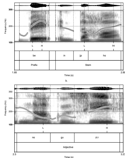
Figure 4: F0 contour of polymorphemic words with single and double rises.
