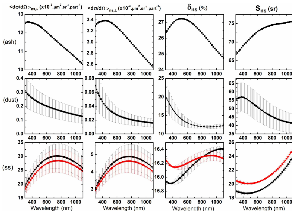
Fig. 4. Ns-particle backscattering coefficients, particle depolarization ratios \delta_{ns} and lidar ratios S_{ns} as a function of the \lambda wavelength, for each ns-particles type: volcanic ash, desert dust and sea salt (ss). The plotted error bars correspond to the size and shape sensitivity study performed in Sect. 3.4. For ss-particles, two curves are represented, one for each refractive index given in Table 2.
