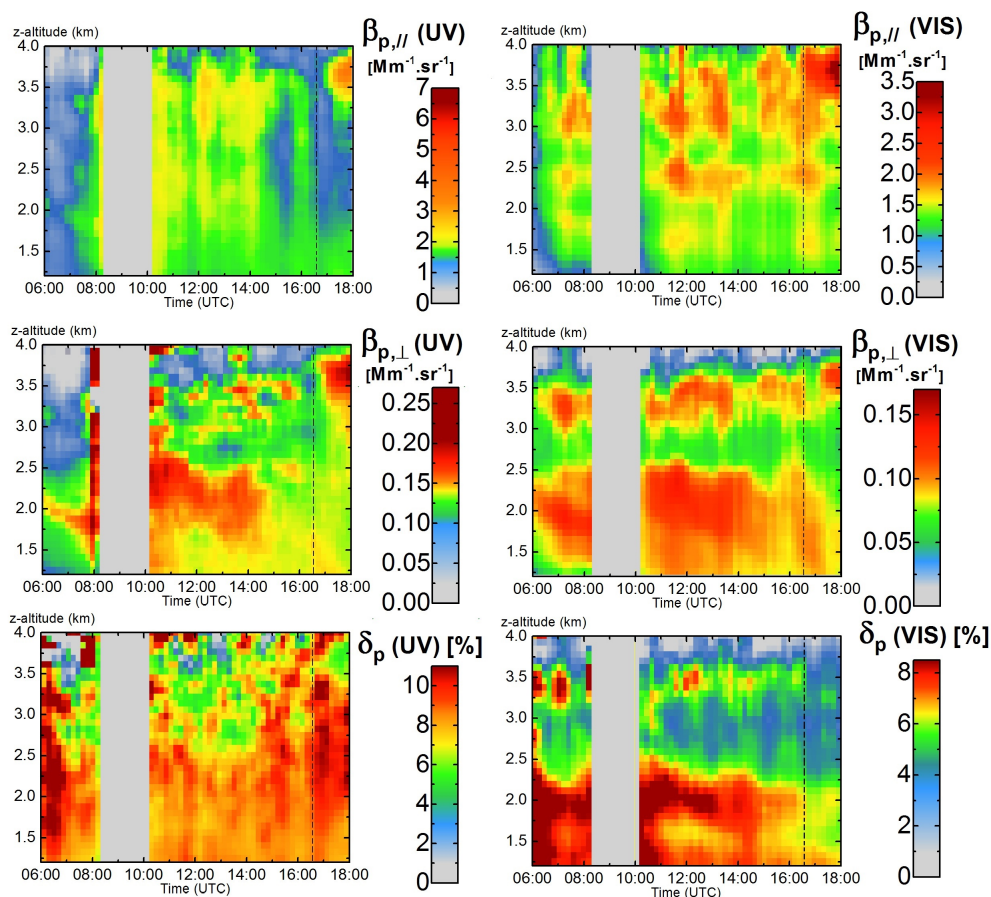
Fig. 9. Time–altitude maps of \beta_{p,\parallel} , \beta_{p,\perp} and \delta_p in the UV ( \lambda_1 = 355 nm, left three panels) and in the VIS ( \lambda_2 = 532 nm, right three panels) on 18 October 2011 at Lyon. The grey band corresponds to clouds which prevented retrieving the \beta_{p,\parallel} , \beta_{p,\perp} , \delta_p coefficients. Dashed lines correspond to Fig. 10, case study at 16:15 UTC.
