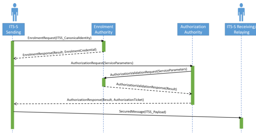
Fig. 3 ITS-S enrolment-authorization process
