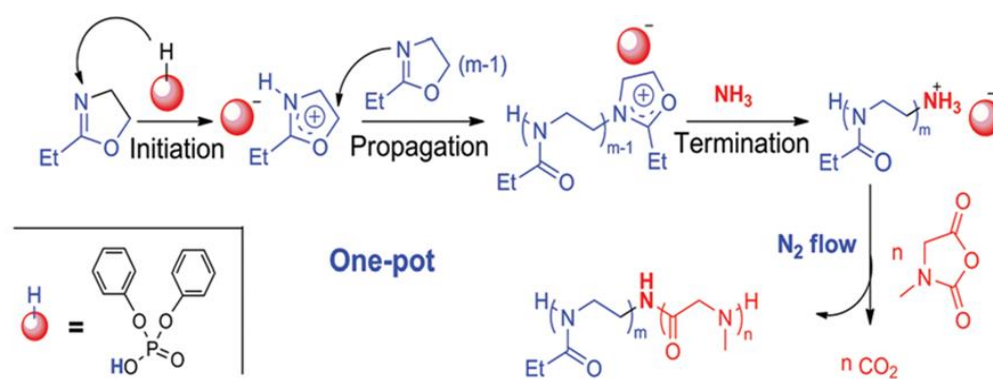
Figure 1. One-pot synthesis of PEtOx- b -PSar diblock copolymers [70].
