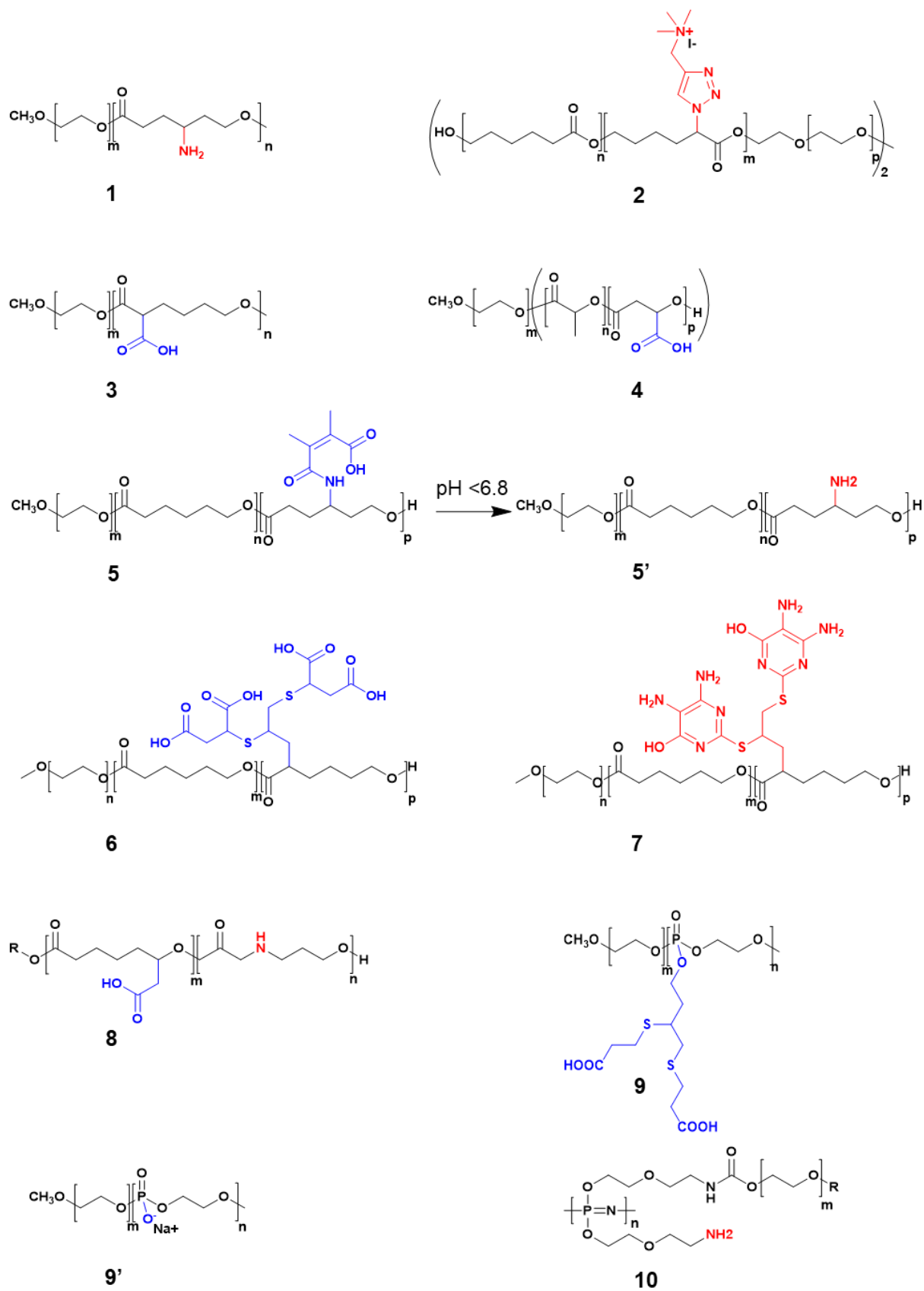
Figure 4. Degradable hydrophilic block copolymers based on polyester, polyphosphoester and polyphosphazene blocks.
