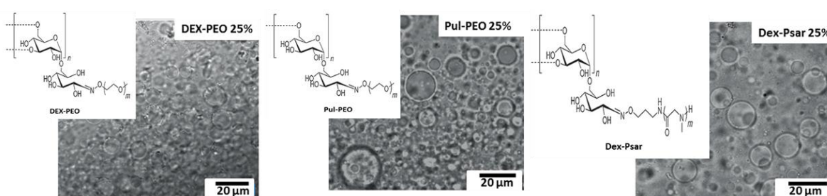
Figure 3. Optical microscopy images of the giant double hydrophilic polymer vesicles referred to as “aquanelles” prepared from Dex- b -PEO, Pul- b -PEO and Dex- b -PSar at 25 wt% (adapted with permission from [65]).
