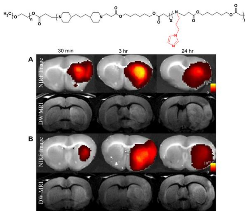
Figure 5. In vivo diffusion-weighted MRI (DW-MRI), near-infrared fluorescence (NIRF) images and signal quantification. In the coronal cross-sectional NIRF images of rat brains of group A (rats injected with PEG-PAE-API-albumin-Cy5.5) (A) and group B (rats injected with albumin-Cy5.5) (B), albumin-Cy5.5 accumulation is clearly visible in the ischemic area of the
