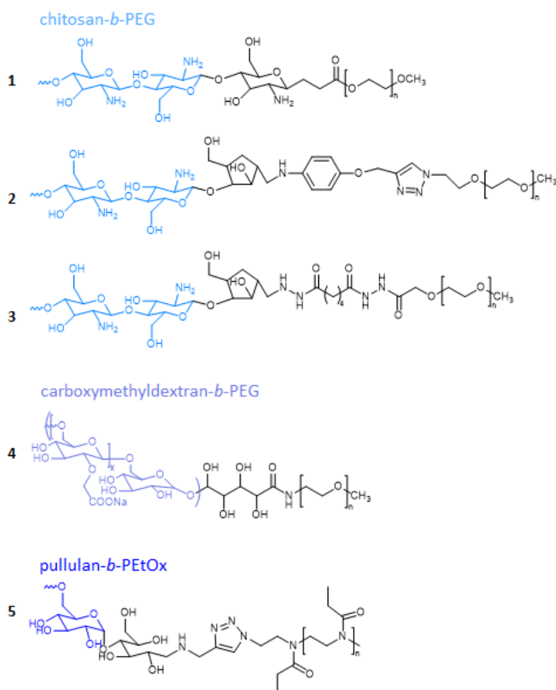
Figure 2. Examples of degradable hydrophilic block copolymers based on polysaccharides.
