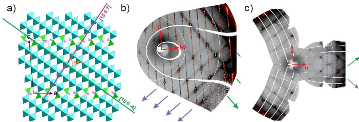
FIG. 1. a) Projection along \mathbf{b} of the structure of \text{Na}_{1.5}\text{P}_4\text{W}_{20}\text{O}_{68} . Blue octahedra are (\text{WO}_6) , green tetrahedra are (\text{PO}_4) and purple circles are Na atoms. The [15\ 0\ 7] and [15\ 0\ -4] directions are showing the short and long direction ( \text{WO}_6 ) chains; they are 90^\circ oriented. b) (0kl)^* c) (hk0)^* planes assembled from the frames collected at 130 K on the ID28 beamline at ESRF[23]. Two directions of diffuse scattering are shown by green and blue arrows. Intensifications of the diffuse signal are observed at the intersection of the two types of diffusion scattering for \frac{1}{2}\mathbf{a}^* (see blue dashed rectangle).
