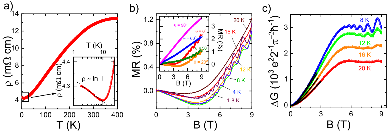
FIG. 3. a) In - plane resistivity versus temperature. Inset: expanded view of the low temperature region shown with logarithmic horizontal scale. Dashed line is a guide for the eye. b) Magnetoresistance as a function of magnetic field applied parallel to c axis. Inset: MR( B ) plots at T = 1.8 K for various \theta angles between the magnetic field direction and the c axis. c) Magnetoconductance versus magnetic field for selected temperatures. The red curves show the data fits with equation (2).
