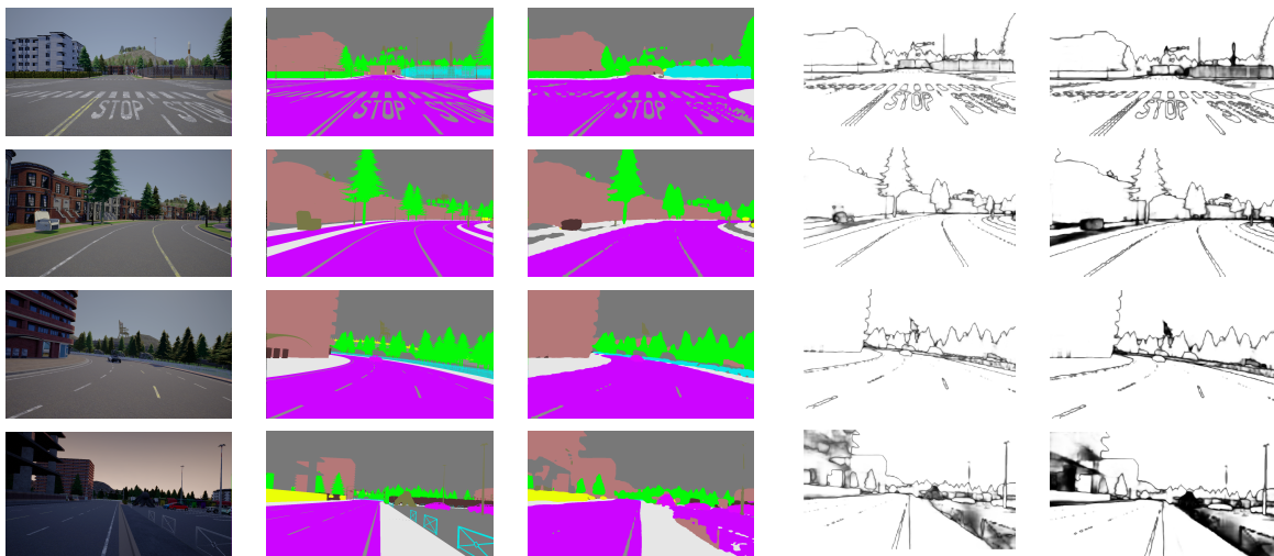
Fig. 7: Results of OVNNI on StreetHazards. The first column is the input image, the second is the ground truth, the third is prediction and the last is the confidence score of OVNNI. For comparison, we add the MCP confidence score in the fourth column. We can see that OVNNI has a low score on the chair, the seat, the rocket and the spider which correspond to the OOD classes.
