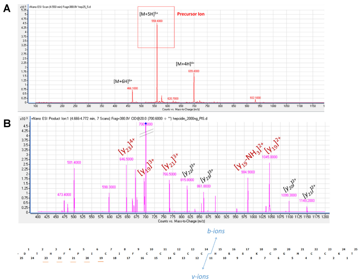
Fig. 1 – (A) Light hepcidin-25 standard chromatograms obtained by nano-HPLC–MS in “full-scan mode” showing quadruply, quintuply and sextuply charged molecular ions. (B) MS/MS spectra of the [M + 5H]^{5+} precursor of light hepcidin-25 standard. In red, the peptide fragment chosen located in the unfolded N termini area of the protein sequence (y19 to y23 ions).
