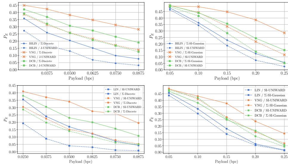
Fig. 7: P_E as a function of payload in bits per coefficients (bpc) for different demosaicking algorithm with the E1Base pipelines. All images are JPEG at QF100. Upper images are steganalyzed with DCTR while lower images were steganalyzed with Efficient-b3.
