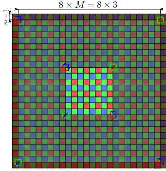
Fig. 2: Dependency structure for a linear pipeline. Due to the use of bilinear demosaicking, adjacent 8 \times 8 block of photo-sites will be correlated after the operation. To be able to take into account all correlations in the DCT domain, a margin of one row/column is necessary at every border of the blocks to compute the correct value of the correlations of the neighboring blocks after demosaicking. Notice that the margin is sufficient because the central block is independent from the block containing the margin.
