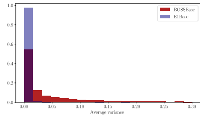
Fig. 16: Histogram of the average variance due to error in modeling content – aka “content” variance – per image for BOSSBase and E1Base.
