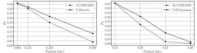
Fig. 13: P_E as a function of the payload in bpc on 5000 noisified images from one BossBase image with the linear processing pipeline. All images are JPEG at QF100.
