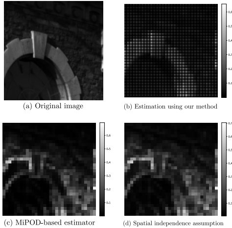
Fig. 3: Comparison of the different structure of the variance maps of the DCT coefficients of image 5105 of the BOSS dataset processed using the linear pipeline (see Table IV) at QF100 depending on the estimation method used. The variance map is either estimated using the method outlined in Section II (upper-right corner) or by assuming pixels to be independent (lower right and lower left). The lower-left figure is obtained by using the variance estimator define in Section IV based on MiPOD’s estimator and propagating the variances in the DCT domain using Eq (29). The lower-right one is obtained using our method to estimate variances in the spatial domain but then foregoing dependencies between pixels by propagating variances in the DCT domain in the same way as for the MiPOD-based estimator.
