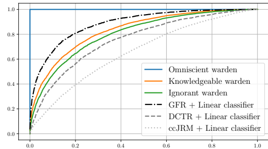
Fig. 5: ROC curves of the LRT for the different types of Warden/models compared with the empirical detector using DCTR and LCLC on 10000 noisified version of the RAW image IMG_3699.cr2 from E1Base. The resulting noise is correlated due to the processing pipeline. Images are compressed with JPEG at QF100 embedded with \Sigma -SI-Gaussian at 0.15bpp.
