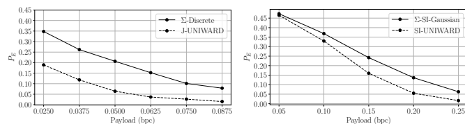
Fig. 8: P_E as a function of payload in bpc for downscaled images on CanonBase with the CanonBase pipelines. All images are JPEG at QF100.
