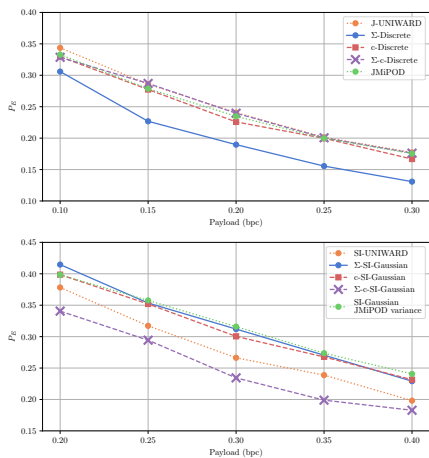
Fig. 12: P_E as a function of payload in bpc for images on Bossbase with the BOSS pipeline comparing the performance of the steganography depending on the variance map used. All images are JPEG at QF100.
