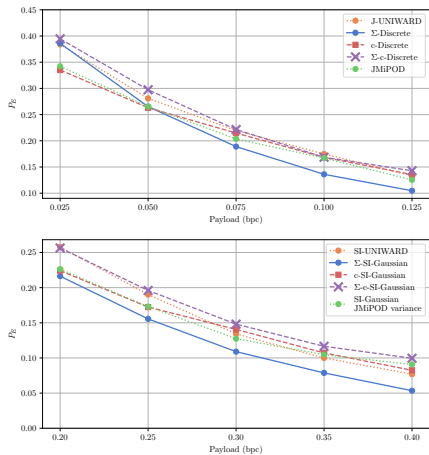
Fig. 11: P_E as a function of payload in bpc for images on Bossbase with the linear processing pipeline comparing the performance of the steganography depending on the variance map used. All images are JPEG at QF100.
