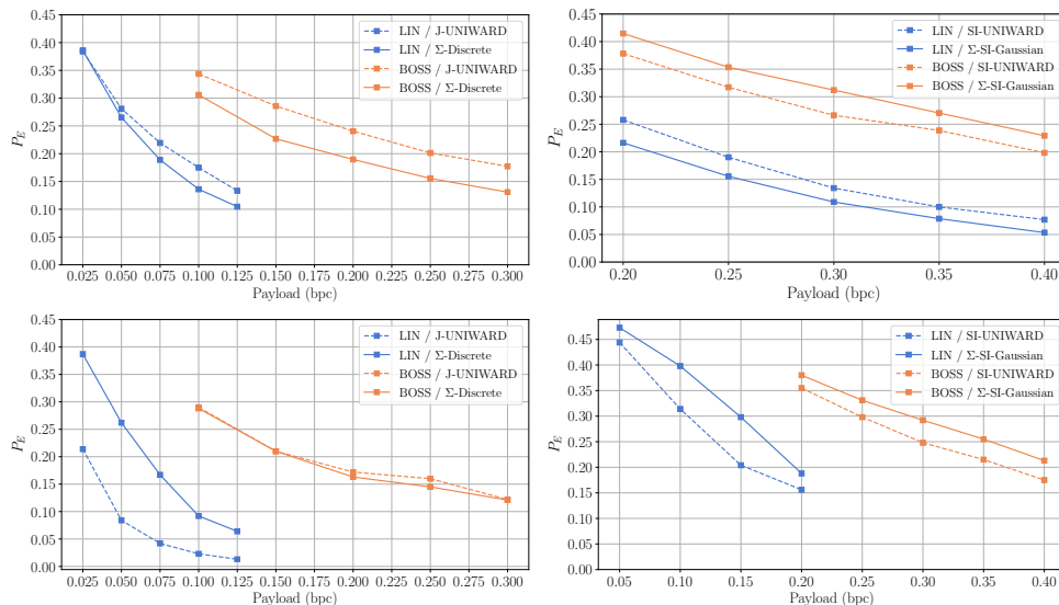
Fig. 10: P_E as a function of payload in bpc for images on Bossbase with two different processing pipeline. The first being the linear processing pipeline, the second being the BOSS pipeline. All images are JPEG at QF100. Steganalysis was performed using DCTR and the LCLC on the upper figures while it was performed with EfficientNet-b3 on the lower ones.
