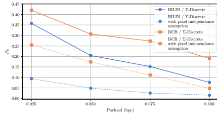
Fig. 14: P_E as a function of payload in bits per coefficients (bpc) on E1Base processed with E1Base pipelines. It compares the variance estimation method when independence is assumed in the spatial domain or in the DCT domain. All images are JPEG at QF100.
