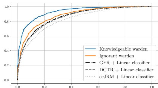
Fig. 6: ROC curves of the LRT for the different types of Warden/models compared with the empirical detector using DCTR and LCLC on 10000 noisified version of the JPEG from IMG_3699.cr2 from E1Base. The resulting noise is independent. Images are compressed with JPEG at QF100 embedded with \Sigma -SI-Gaussian at 0.15bpp.
