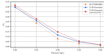
Fig. 15: P_E as a function of payload in bits per coefficients (bpc) on E1Base processed with E1Base pipeline with bilinear demosaicking and gamma correction. All images are JPEG at QF100.
