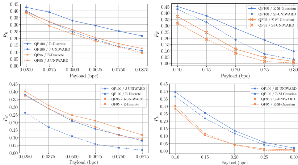
Fig. 9: P_E as a function of payload in bpc for different JPEG quality factors (QF) with CanonBaseQF pipelines. Upper images are steganalyzed with DCTR while lower images were steganalyzed with Efficient-b3.
