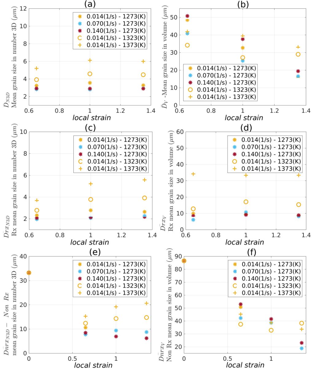
Figure 7: Evolution of \bar{D}_{N3D} (a,c,e) and \bar{D}_V (b,d,f) as a function of strain, considering all the grains (a,b), the recrystallized grains (c,d) and the non recrystallized grains (e,f) for the different deformation conditions.
