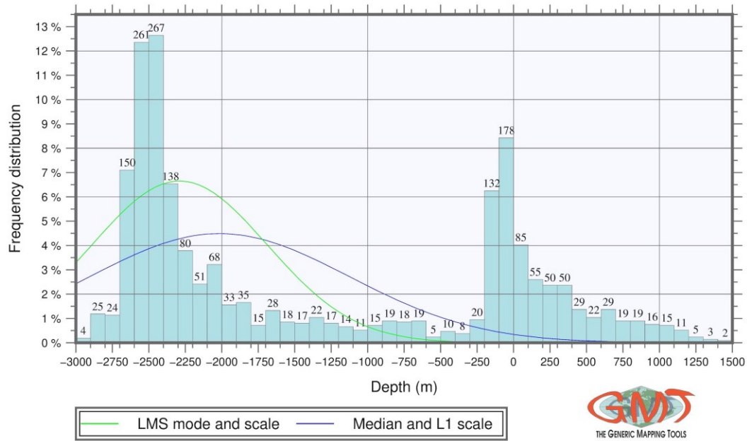
Fig. 7 Depth distribution in the Cascadia Subduction Zone west of Vancouver Island
