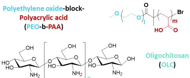
Fig. 1. Chemical structure of PEO- b -PAA DHBC and OC
