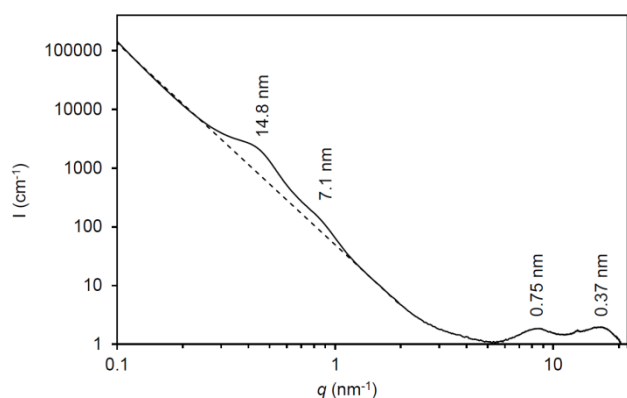
Fig. 4 SAXS and WAXS profile of unwashed PICPMO
