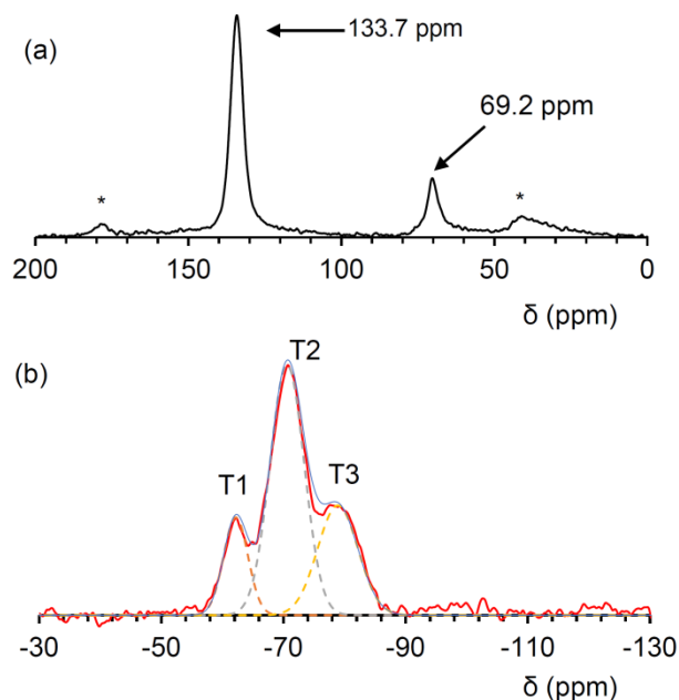
Fig. 5 (a) 13 C CPMAS and (b) 29 Si MAS NMR spectra of washed PICPMO
