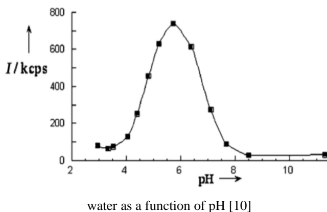
Fig. 2. Scattered light intensity of OC and PEO- b -PAA in
