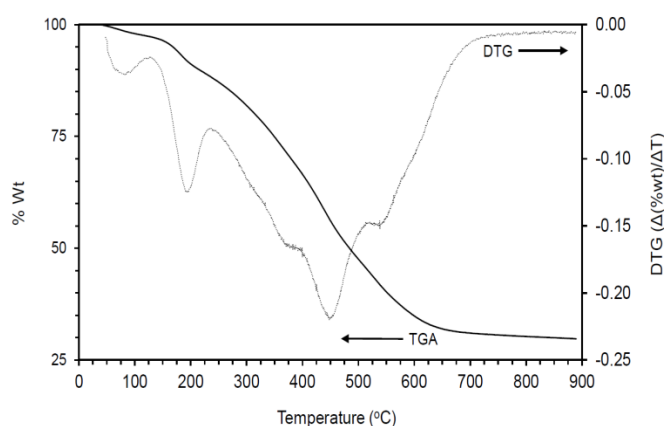
Fig. 7 Thermogravimetric analysis of as-prepared PICPMO material (containing template)
