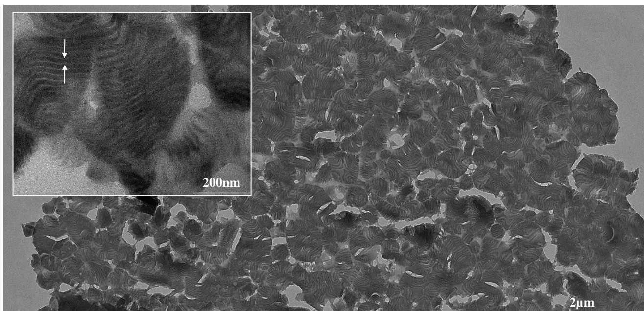
Fig. 3 Transmission Electron Microscopy of the lamellar mesostructured hybrid PICPMO
