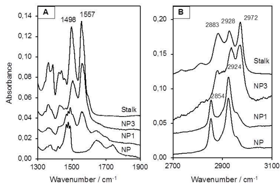
Figure 4. IR spectra (A) from 1300 to 1900 \text{cm}^{-1} and (B) from 2700 to 3100 \text{cm}^{-1} of NPs and the Stalk precursor
