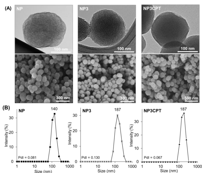
Figure 7. (A) TEM and SEM images and (B) DLS measurements of NP , NP3 and NP3CPT , nanomaterials. The polydispersity indices (Pdl, measured by DLS) are included.
