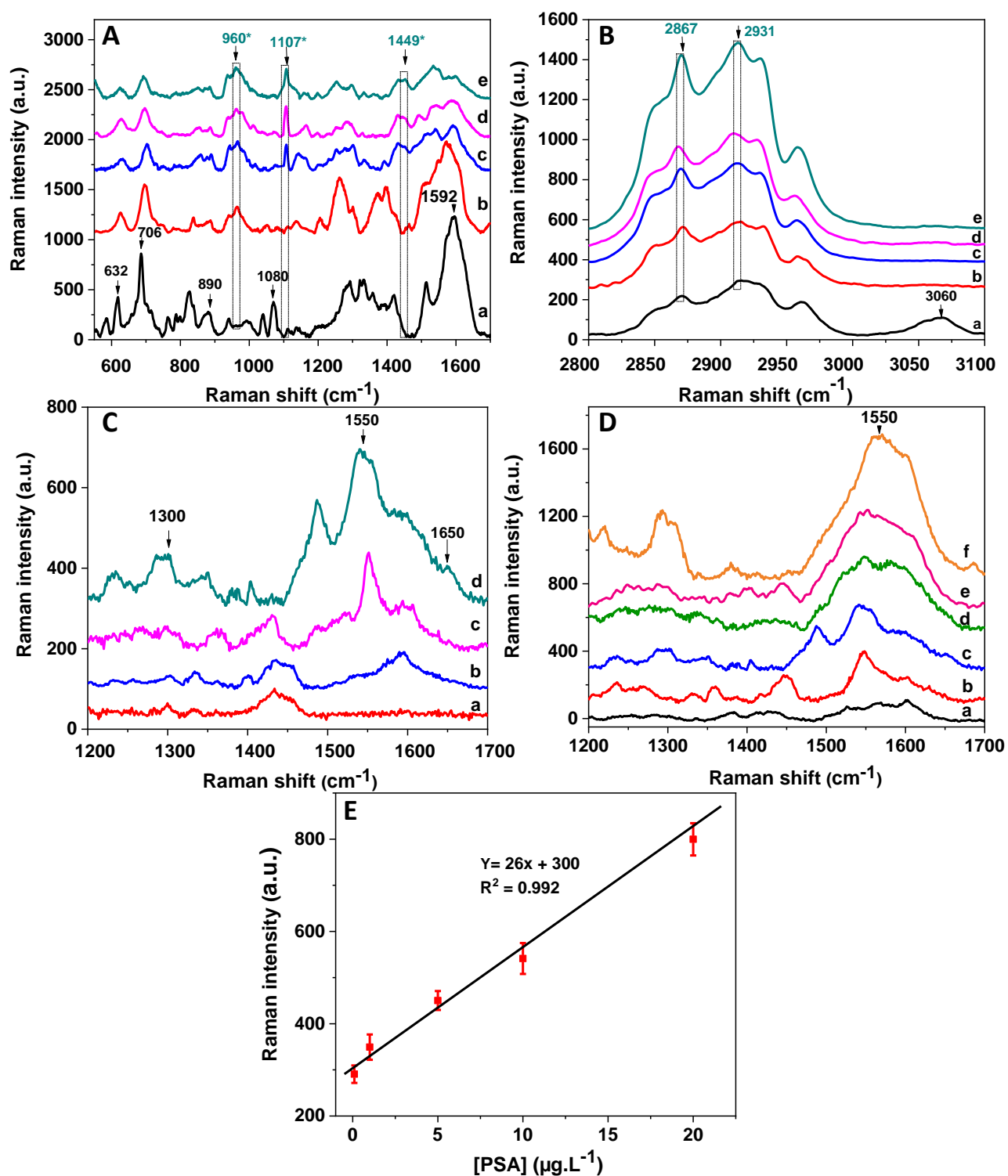
Figure 3. Raman spectra of MCH/AgNPs/SiNWs (a) and anti-PSA/MCH/AgNPs/SiNWs for different incubation times in aptamer ; 4h (b), 8h (c), 12h (d) and 16h (e) for two frequency ranges: 550-1700 \text{cm}^{-1} (A) and 2800-3100 \text{cm}^{-1} (B). Raman spectra of PSA(1 \mu\text{g.L}^{-1} )/anti-PSA/MCH/AgNPs/SiNWs for different incubation times ; 4h (a), 8h (b), 12h (c) and 16h (d) of the SERS substrate
