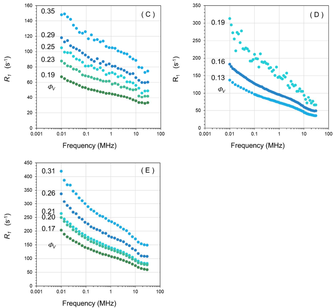
Figure 2 : ^1\text{H} relaxation rate R_1 dispersion profile of water in several GE dispersions for several pigment volume fraction: (A) Cyprus GE, (B) Cyprus GBE, (C) Russia GE, (D) France GE and (E) Sennelier GE.
