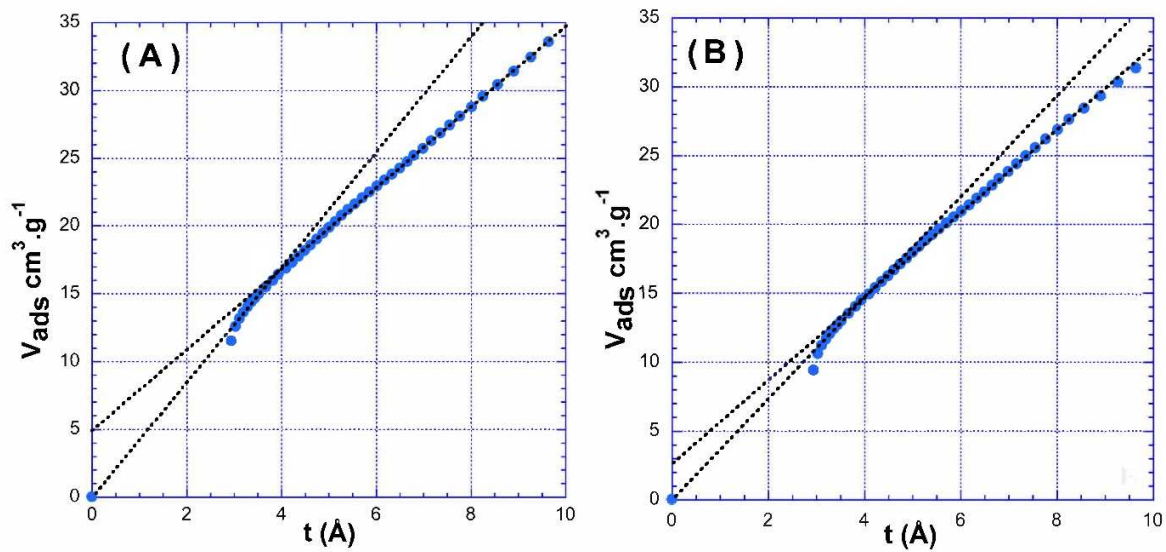
Figure 4 : t-plot curves obtained for Bohemian GE (A) and Cyprus GE (B).
