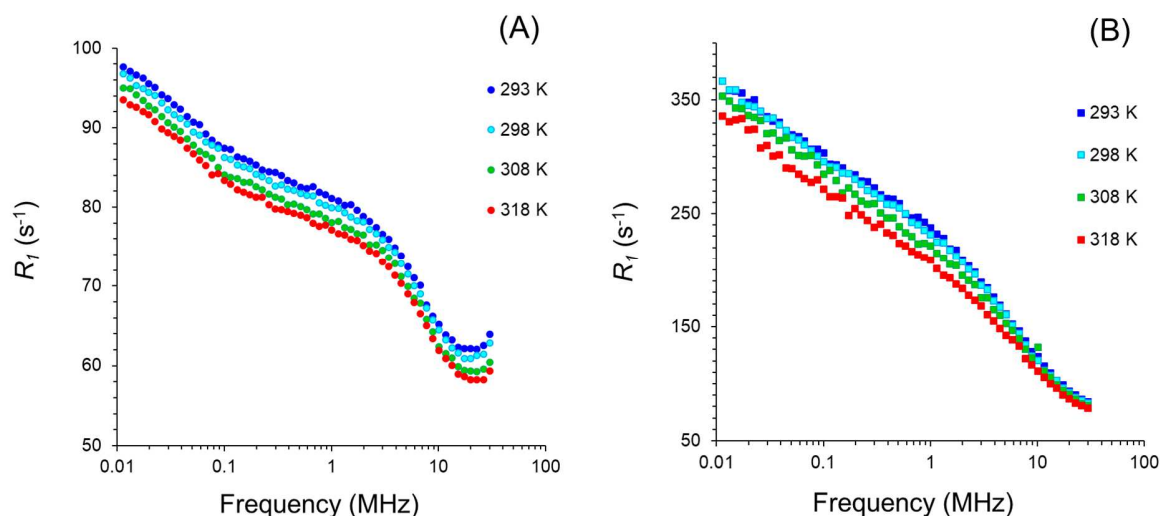
Figure 5 : ^1\text{H} NMR relaxation profile for Bohemian GE (A) and Cyprus GE (B) at 293K (blue), 298K (cyan), 308K (green) and 318K (red).
