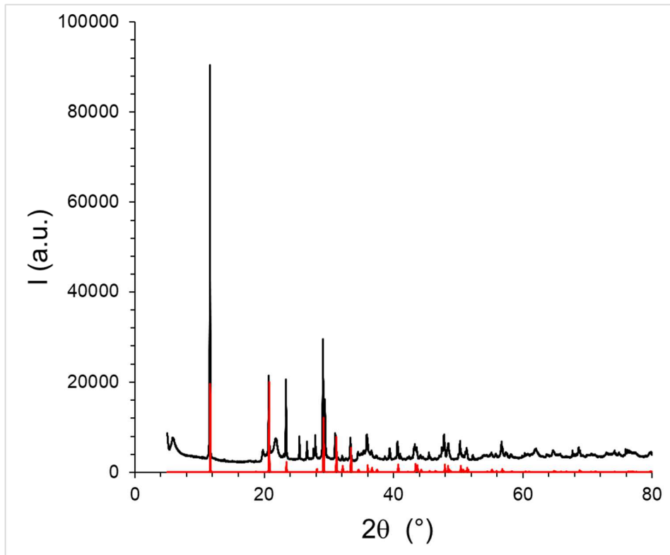
Figure 1 : XRD pattern of France GE powder (black) and calculated XRD pattern of \text{CaSO}_4 \cdot 2\text{H}_2\text{O} from the CIF file [2].
