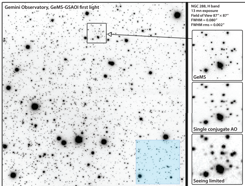
Fig. 1. Figure illustrating the gain in FoV brought by MCAO with NGC 288 observed by GeMS in the H band. Figure extracted from Rigaut & Neichel (2018)
