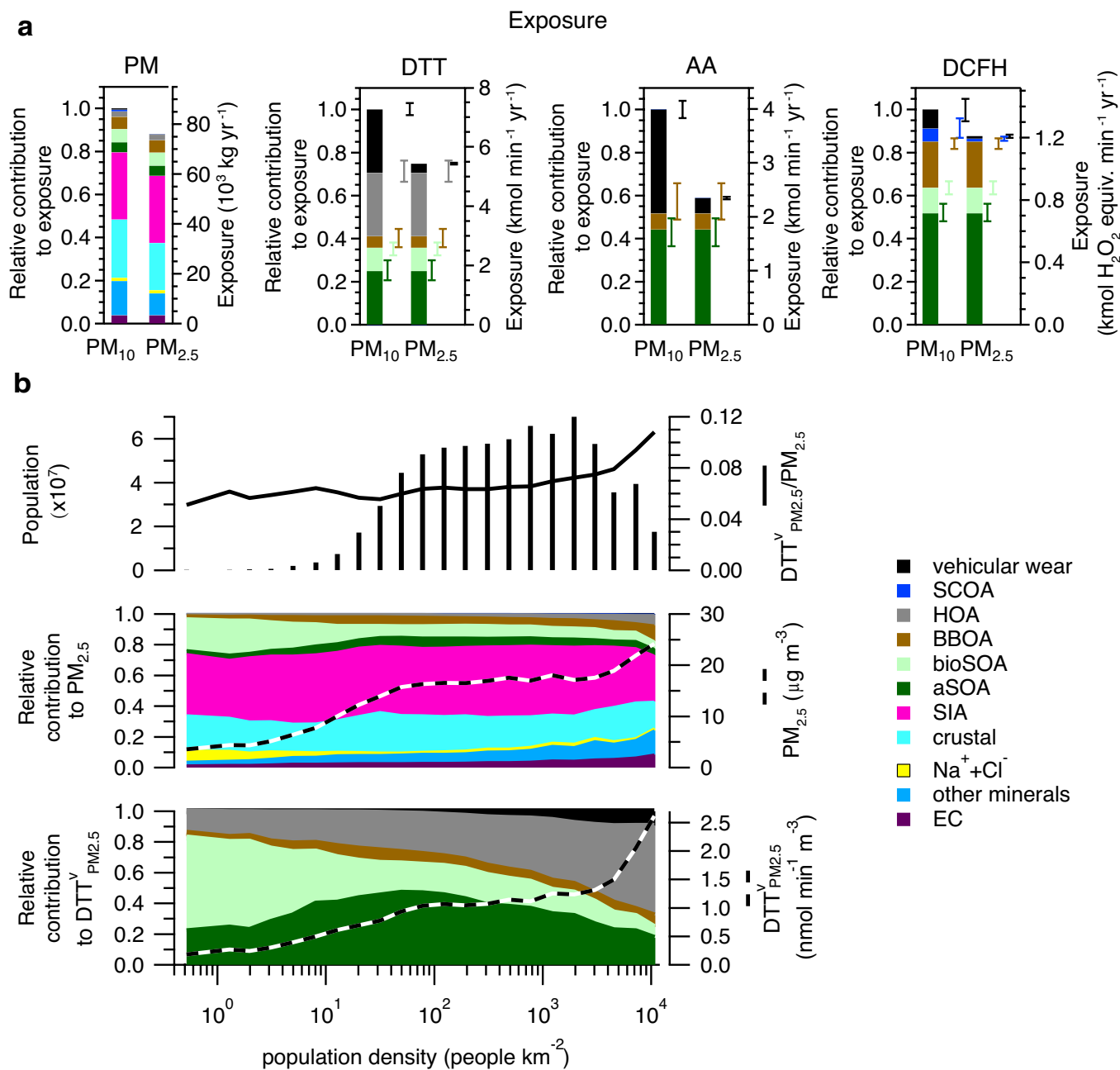
Extended Data Fig. 8 | Source contributions to PM and OP exposure, and their dependence on population density for \text{PM}_{2.5} and \text{OP}_{\text{PM}_{2.5}}^v .
