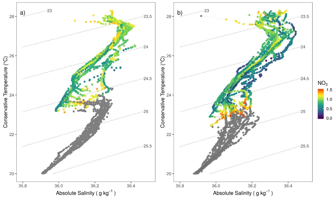
Figure 6: TS diagrams issued from FLeeT during (a) period 2 and (b) period 3 as defined in Section 3.3.1. Black dotted lines represent isopycnal surfaces (interval= 0.5 kg m -3 ). Colours refer to NO 3 - concentrations (μmol kg -1 ). NO 3 - higher than 1.5 μmol kg -1 are in grey.
