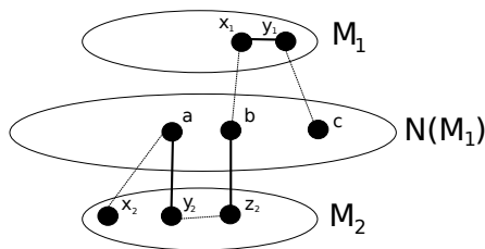
Figure 5: An augmenting path of length 7 with ends x_2, c . Matched edges are drawn in bold.
