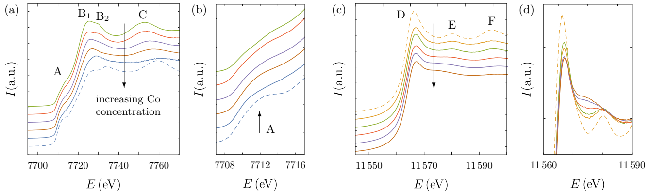
FIG. 2. XANES data obtained at the Co K- and Pt L_3 -edges (increasing Co concentration from top to bottom) and main features labeled from A to F: Co and Pt foil (dashed blue and dashed orange, respectively) and samples S7 (blue), S6 (brown), S4 (purple), S2 (red), S1 (green) and S0 (orange). (a) Co K-edge, (b) magnified spectra illustrating the decreasing magnitude of peak A with increasing Pt concentration. (c) Pt L_3 -edge and (d) zoom on the white line. Note that the curves in (a-c) were shifted vertically for clarity.
