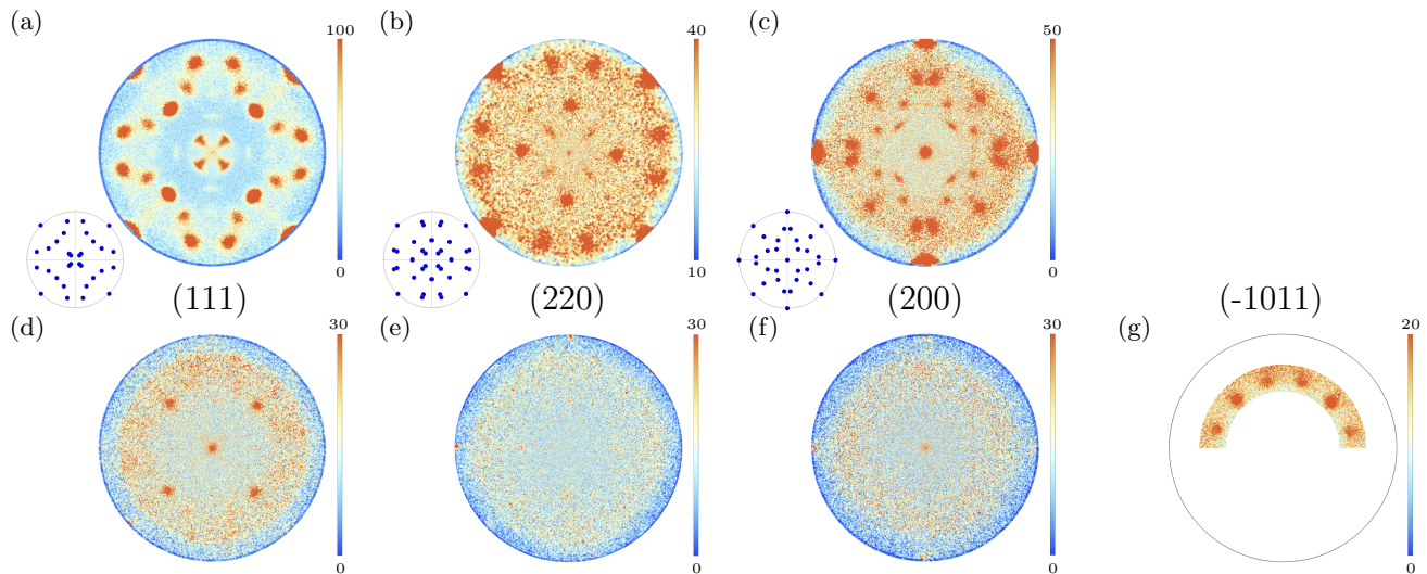
FIG. 6. Pole figure measurements. (a-c) (111), (220) and (200) poles in a Pt-rich sample (S1) as well as predictions using three different crystallite orientations (inset). (d-g) (111), (220) (200) and (-1011) poles in a Co-rich sample (S4).
