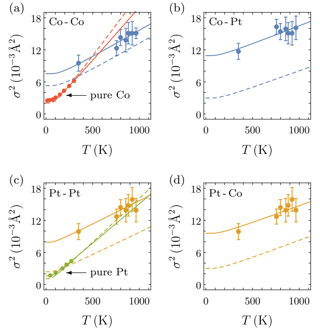
FIG. 5. Evolution of the Debye-Waller EXAFS parameter \sigma^2 with temperature. Measurements performed at the (a-b) Co K edge (blue) and (c-d) Pt L 3 edge (orange) as well as literature data gained on pure Co and Pt systems (red and green) and fits to eq.1 (fits to MEAM simulations: dashed lines, fits to experimental data: solid line).
