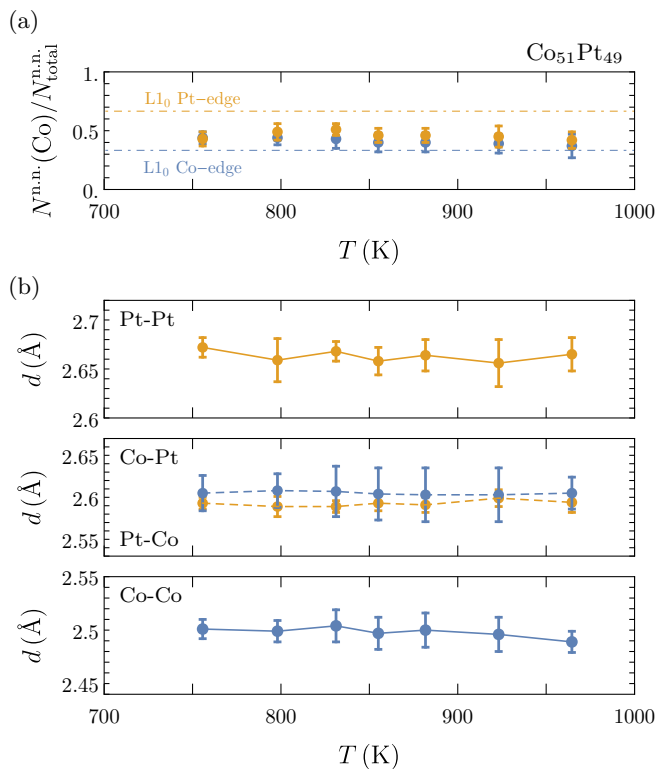
FIG. 4. In situ annealing study performed on sample S3, using annealing times t_a^* = 10\text{h} (at 750 K) and t_a = 2\text{h} for all other temperatures. (a) Local Co (n.n) concentration (blue dots: Co K-edge, orange dots: Pt L 3 edge, dashdotted lines: expected values for an ideal L1 0 phase) and (b) n.n distances as a function of T (same color coding as before).
