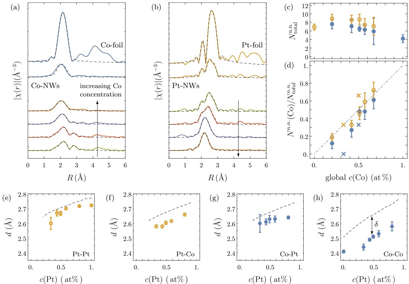
FIG. 3. EXAFS measured on nanocolumnar CoPt-SrTiO 3 samples with varying Co/Pt ratio (arrows indicate increasing Co concentrations). Co and Pt foil data are shown for comparison. \chi(r) data obtained after Fourier transformation of k^2\chi(k) at the (a) Co K-edge and (b) Pt L 3 -edge (same color coding as in Fig.2) as well as corresponding fits (black dashed line). (c) Total number of next neighbors (n.n.) as a function of concentration, (d) local Co concentration vs global Co concentration (crosses indicate the values expected for pure L1 0 and L1 2 phases), n.n. distances for (e) Pt-Pt, (f) Pt-Co, (g) Co-Pt and (h) Co-Co bonds (blue solid points: Co K-edge, orange circles: Pt L 3 -edge, black dashed line: MEAM results).
