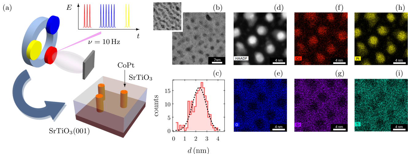
FIG. 1. Schematics of the growth procedure and exemplary electron microscopy data. (a) Sequential pulsed laser deposition using Pt, CoO and SrTiO 3 targets, results in growth of CoPt–SrTiO 3 nanocomposites. (b) HR-TEM plan view and tilted view, which unravels the columnar morphology of the nano-inclusions in the single crystal SrTiO 3 matrix. (c) Diameter distribution of the embedded structures (sample S4) (d-i) plan view STEM-HAADF and EDX data (sample S1) provide detailed chemical information on the nanocomposite and confirm phase separation and creation of CoPt nanoalloys.
