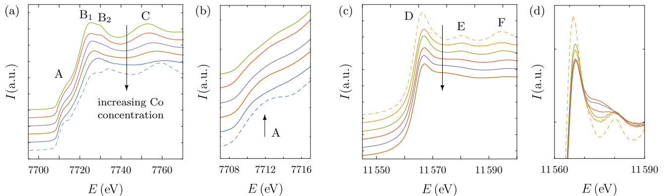
FIG. 2. XANES data obtained at the Co K- and Pt L_3 -edges (increasing Co concentration from top to bottom) and main features labeled from A to F: Co and Pt foil (dashed blue and dashed orange, respectively) and samples S7 (blue), S6 (brown), S4 (purple), S2 (red), S1 (green) and S0 (orange). (a) Co K-edge, (b) magnified spectra illustrating the decreasing magnitude of peak A with increasing Pt concentration. (c) Pt L_3 -edge and (d) zoom on the white line. Note that the curves in (a-c) were shifted vertically for clarity.
