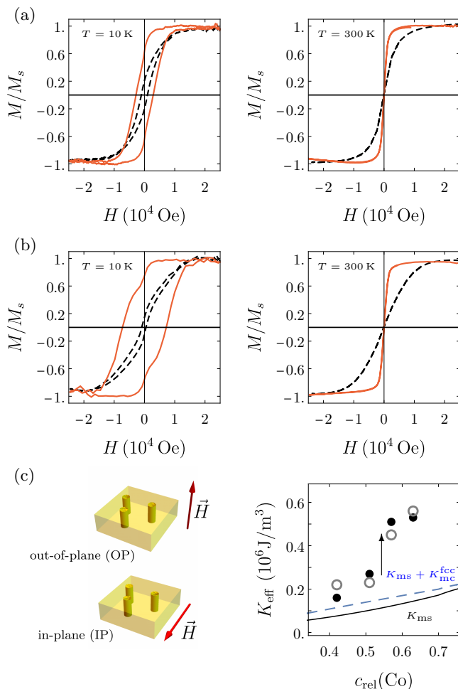
FIG. 7. Temperature dependent magnetometry measurements: (a) At 10 K (left) and 300 K (right) in IP (black, dashed line) OP geometries (red, solid line) below c_{\text{crit}} (sample S3) and (b) At 10 K (left) and 300 K (right) in IP (black, dashed line) OP geometries (red, solid line) above c_{\text{crit}} (sample S5). (c) IP and OP measurement geometries employed in this work (left). Effective uniaxial anisotropy K_{\text{eff}} calculated from the magnetization loops at 10 K (gray circles) and 300 K (black dots). The magnetostatic anisotropy K_{\text{ms}} (black solid line) and magnetocrystalline K_{\text{mc}} fcc contributions (blue dashed curve) are shown as well (right).
