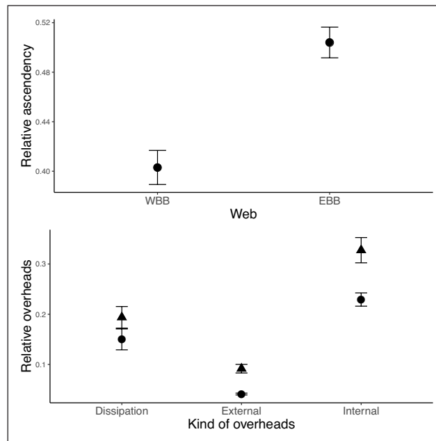
Figure 7: Relative ascendancy and reserves associated with each kind of overheads for both food webs. Relative ascendancy (upper panel) and relative reserves or overheads (lower panel) for both the western Baffin Bay (WBB) food web (triangles) and eastern Baffin Bay (EBB) food web (circles). Relative overheads correspond to overheads scaled by the maximal possible ascendancy. Each symbol represents the mean value with its standard deviation calculated from the set of 20,000 random flows solutions. DOI: https://doi.org/10.1525/elementa.397.f7
