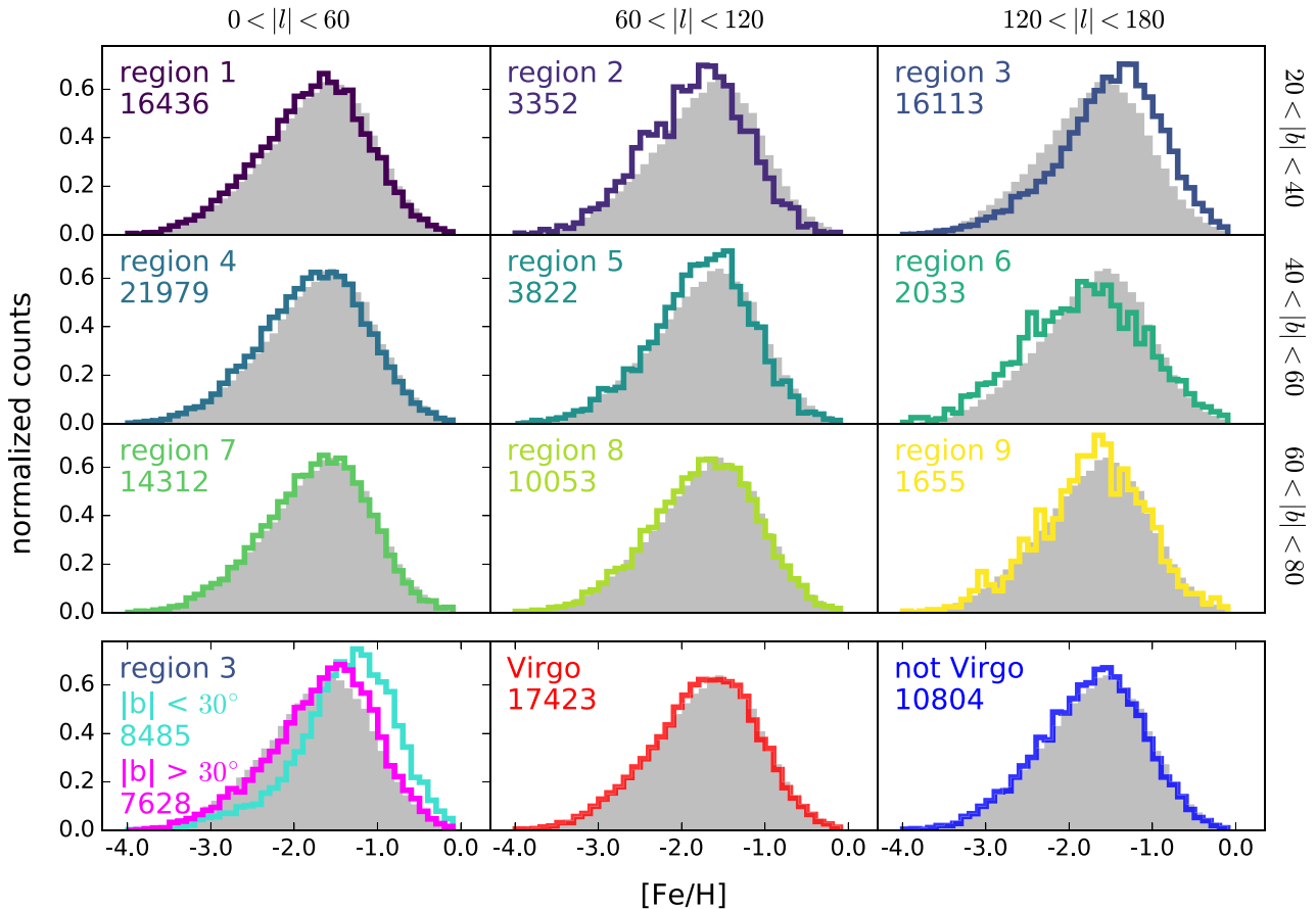
Figure 10. MDFs for the nine different regions described in the text, with colours that correspond to the numbered regions depicted in Fig. 8. The grey-filled histogram is the MDF of the total, GMM corrected halo sample for comparison. The bottom left-hand panel shows the MDFs for region 3, separated into a high- and low-latitude sample (fuchsia and cyan, respectively), and the other two panels in the bottom row show the region selected to contain Virgo in red (the selected region is outlined in Fig. 8), and the rest of the stars at the same Galactic latitude as a comparison are shown in blue.
