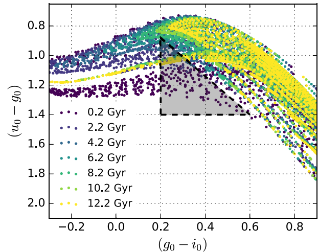
Figure 3. Colour–colour plot of PARSEC isochrones sampling ages of 0.2–12.2 Gyr and metallicities of -2.5 < [\text{Fe}/\text{H}] < -0.5 . The isochrones are coloured by age, but if instead they were coloured by metallicity, the metal-poor populations would be at the top of the plot and the metal-rich ones at the bottom. The grey-shaded triangle shows the region removed (see text for details), which targets young disc stars and old horizontal branch stars.
