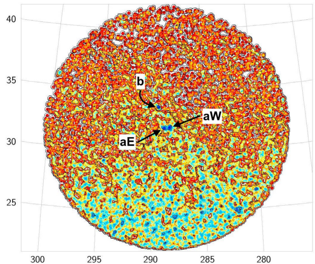
Figure 2. Density map (Galactic coordinates, logarithmic scale) of stars from Gaia DR2 in the region surrounding PW 1. Stars in this map are selected to have proper motion within 1.0 \text{ mas yr}^{-1} from the mean motion of PW 1 and in parallax, to reject obvious nearby stars. The three components of the stellar system are indicated by the arrows and are labelled.
