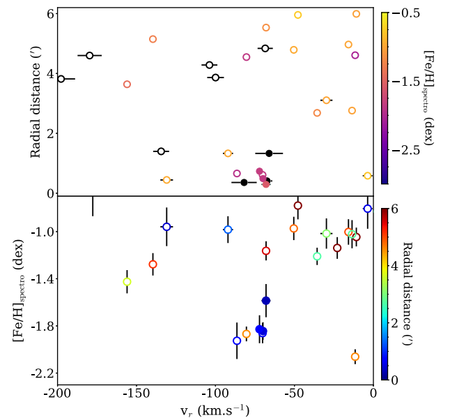
Figure 5. Heliocentric velocities versus radial distances (top panel) and spectroscopic metallicities (bottom panel). The coloured circles are non-HB stars with a S/N greater than 10, for which we are able to derive the spectroscopic metallicities. The colour maps stand for the metallicity (top) and radial distance (bottom). The spectroscopic members are shown as the filled dots.
