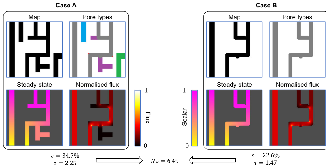
Fig. 2 Illustration of different types of pores that can be present within porous electrodes and their effects on the tortuosity factor \tau and McMullin number N_M determination. The simulated steady-state scalar distributions are shown as well as the normalized flux maps. Case A: microstructure with five different pore types: gray—through pores; blue—dead-end pores for eRDM, that may or may not be available for eSCM, depending on the orientation of the CV; purple—dead-end pores for eRDM that branch from the through pores; green—dead-end pores like Blue but could become through pores if the CV was larger as it extends out the side of the CV; and red—small corner regions having low flux. Case B: microstructure with only through-pores (gray) based on low flux threshold. The microstructure size is 256 \times 56 pixels.
