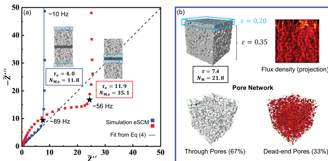
Fig. 6 Illustration of a numerically generated 3D microstructure having two adjacent layers with two different porosities. 90% of volume has \varepsilon = 35\% , while 10% (cyan box) of volume has \varepsilon = 20\% . a The plot shows the simulated EIS of eSCM along with the fit using Eq. 4. The plot contains an inset showing the cross-section of the two microstructures, that have either the lower porosity region at the current collector side (blue square) or at the separator side (red square), in symmetric cell configuration with the associated electrode tortuosity factor \tau_e ; b The 3D microstructure that has lower porosity at the top is shown in detail along with the associated tortuosity factor \tau given by eRDM simulation. The simulated flux density shows a lower density on the top corresponding with the lower porosity region. The pore network separated in through-pores and dead-end pores is also presented. The microstructure size is 50 \times 50 \times 50 voxels, the voxel size equals to 1 \mu\text{m} .
