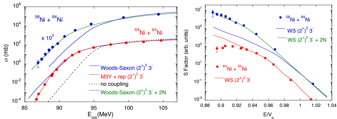
Figure 2. (left panel) Fusion excitation function of ^{58}\text{Ni} + ^{64}\text{Ni} (blue dots) and ^{64}\text{Ni} + ^{64}\text{Ni} (red dots), compared with CC calculation, see text. (right panel) S -factor for ^{58,64}\text{Ni} + ^{64}\text{Ni} compared to CC calculations using a WS potential.
