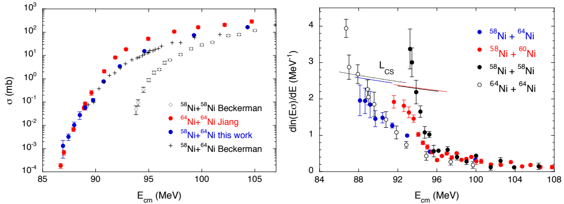
Figure 1. (left) Fusion excitation functions for Ni + Ni systems from the present and previous measurements, see text for details. (right) Logarithmic derivatives for several Ni + Ni systems.
