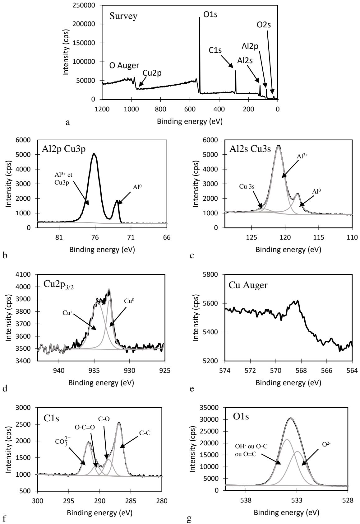
Figure 5 : XPS spectra recorded on AlCu 2.2 at % sample a) Survey spectrum b) Al 2p and Cu 3p core level spectrum c) Al 2s and Cu 3s core level spectrum d) Cu 2p 3/2 core level spectrum e) Cu Auger spectrum f) C1s core level spectrum g) O1s core level spectrum.
