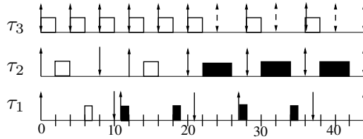
Fig. 4. FP Scheduling of \tau_1 using AFM and policy_1
