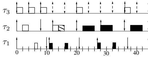
Fig. 3. FP Scheduling of \tau_1 using AMC
