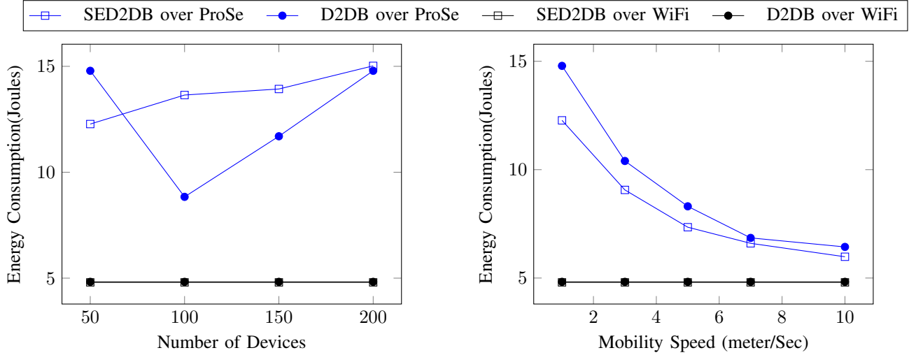
Fig. 4: Energy consumption vs Number of Devices
