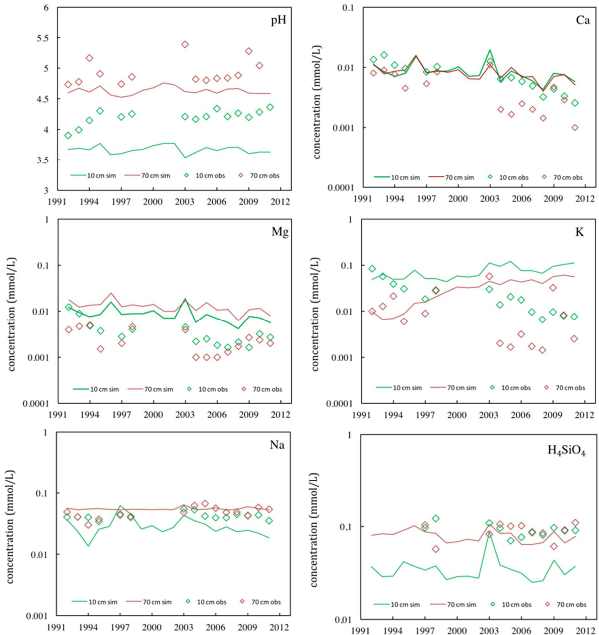
Figure 4: Mean annual pH and concentration of major cations (mmol/L) and H 4 SiO 4 (mmol/L) as a function of time on the HP site. Dots stand for data acquired on the lysimetric plates (at 10 cm in green and at 70 cm in red) and solid line is the model output (at 10 cm in green and at 70 cm in red).
