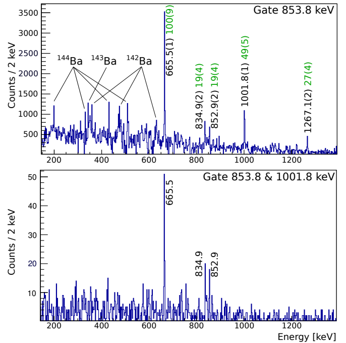
Figure 2. Upper panel: Background-subtracted energy spectrum coincident to the gate on the 853.8 keV 4_1^+ \rightarrow 2_1^+ transition in the prompt time window. The efficiency-corrected intensities normalized to the strongest transition at 665.5 keV (green) are shown next to the peaks. Only events where at least three different HPGe detector hits were recorded are considered. Lower panel: The energy spectrum after a second gate on 1001.8 keV is applied.
