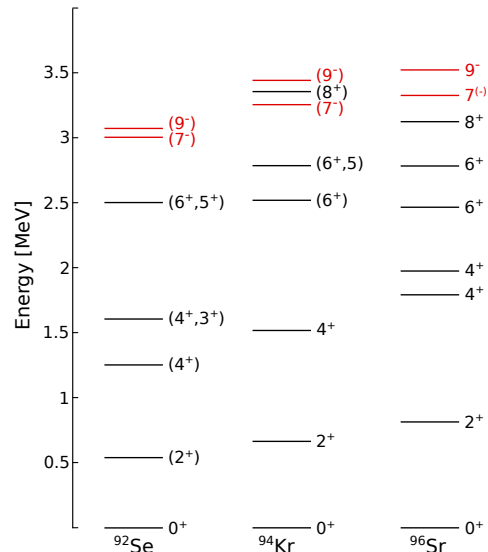
Figure 10. Comparison of partial level schemes of ^{92}\text{Se} , ^{94}\text{Kr} , and ^{96}\text{Sr} . Data from this work and Ref. [18, 33, 35, 36].
