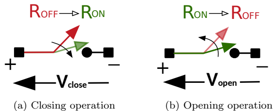
Figure 5: Memristor Behavioral Model
