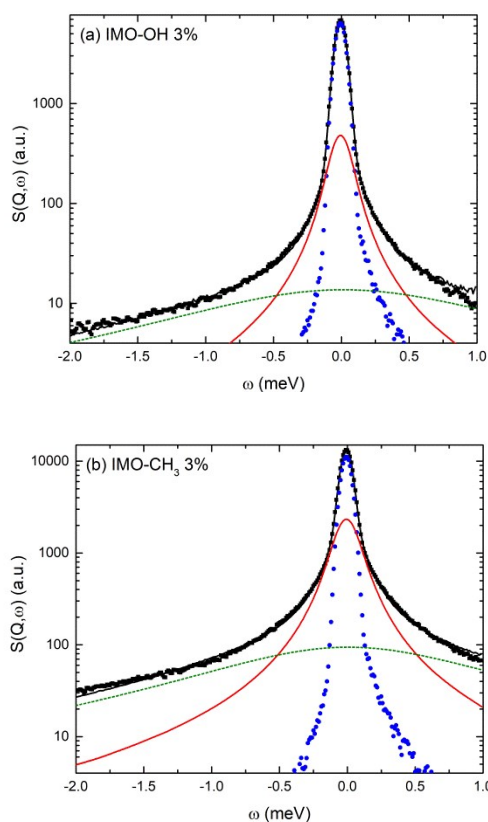
Fig. 5 Example of fitting procedure for the quasi-elastic spectra measured for a) IMO-OH and b) IMO-CH 3 . Both samples are equilibrated at 3% RH. In both cases, Q = 1.75 \text{ \AA}^{-1} . Black dots: Experimental data; Black line: Fit; Blue dots: Resolution function; Red solid line: Narrow Lorentzian; Green dotted line: Broad Lorentzian.
