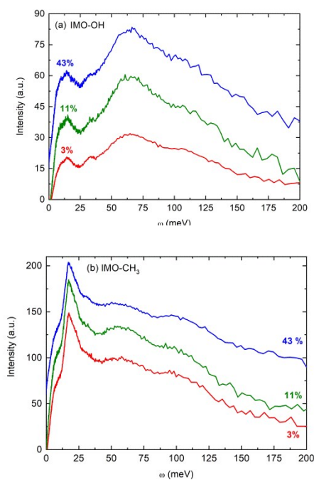
Fig. 2 Vibrational density of states: a) IMO-OH samples; b) IMO-CH 3 samples at all three studied RH values (3% in red, 11% in green and 43% in blue). Intensities are not normalized. The curves are shifted with respect to each other, as only the positions of the bands are discussed in the text. The temperature was 295 K.
