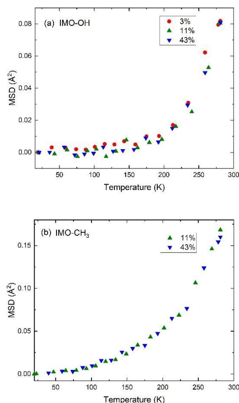
Fig. 4 Evolution of MSD as a function of temperature in a) IMO-OH samples; b) IMO-CH 3 samples. The RH values at which the samples are equilibrated, are indicated. MSD is expressed in Å 2 and reduces to \langle u^2 \rangle / 3 at low temperature.
