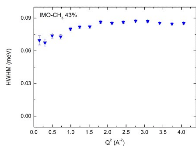
Fig. 7 HWHM of the narrow component plotted versus Q^2 , for the IMO- \text{CH}_3 sample equilibrated at 43% RH.
