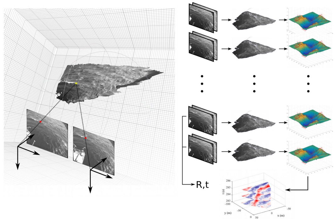
Fig. 3 Left: 3-D surface points can be estimated by triangulating exiting rays passing through corresponding image points. Right: wave field estimation process. A subset of the stereo frames are used to compute the extrinsic parameters ( \mathbf{R}, \mathbf{T} ) necessary to create a dense 3-D point cloud for each stereo-pair. Each point cloud is interpolated in a regular surface grid and a spatio-temporal wave field is obtained by stacking all the reconstructed surfaces.
