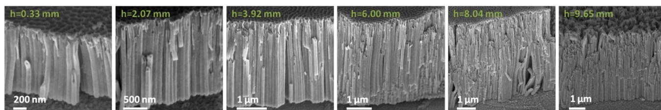
Figure 2 : SEM images of TiO 2 -NTs observed at different height of the nanotubes (observed with a tilt angle of 45°).
