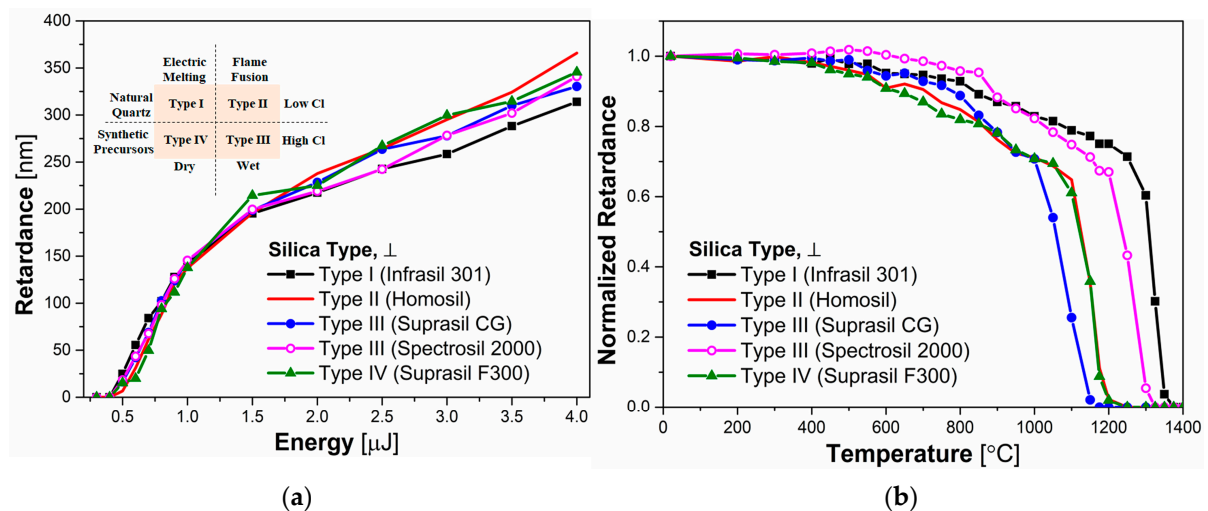
Figure 3. (a) Retardance as a function of pulse energy for \text{SiO}_2 glasses: Type I (Infrasil 301 ® ), II (Homosil ® ), III (Suprasil CG ® and Spectrosil 2000 ® ), and IV (Suprasil F300 ® ). Laser parameters are: 1030 nm, 250 fs, 100 kHz, 100 \mu\text{m/s} , NA = 0.6, laser polarization \perp to writing direction. Inset: category and characteristics of sample; (b) Normalized retardance ( R_{norm} ) as a function of temperature for all \text{SiO}_2 glasses. Pulse energy is 2 \mu\text{J} /pulse and other laser conditions are same mentioned above. The measurements were performed at room temperature.
